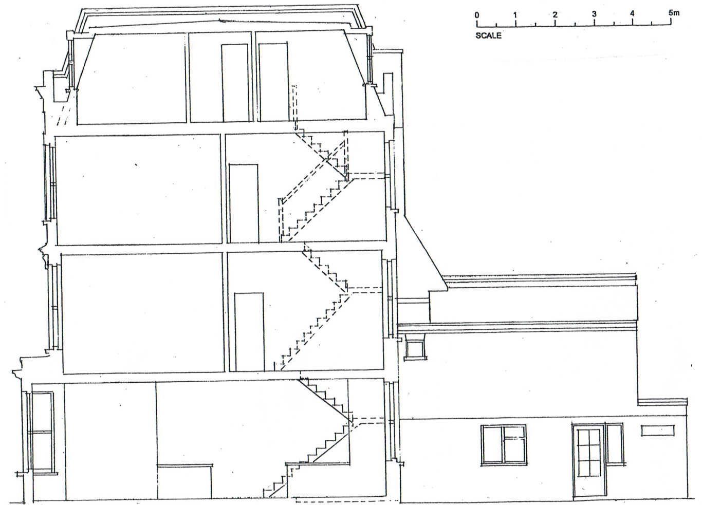
Section
