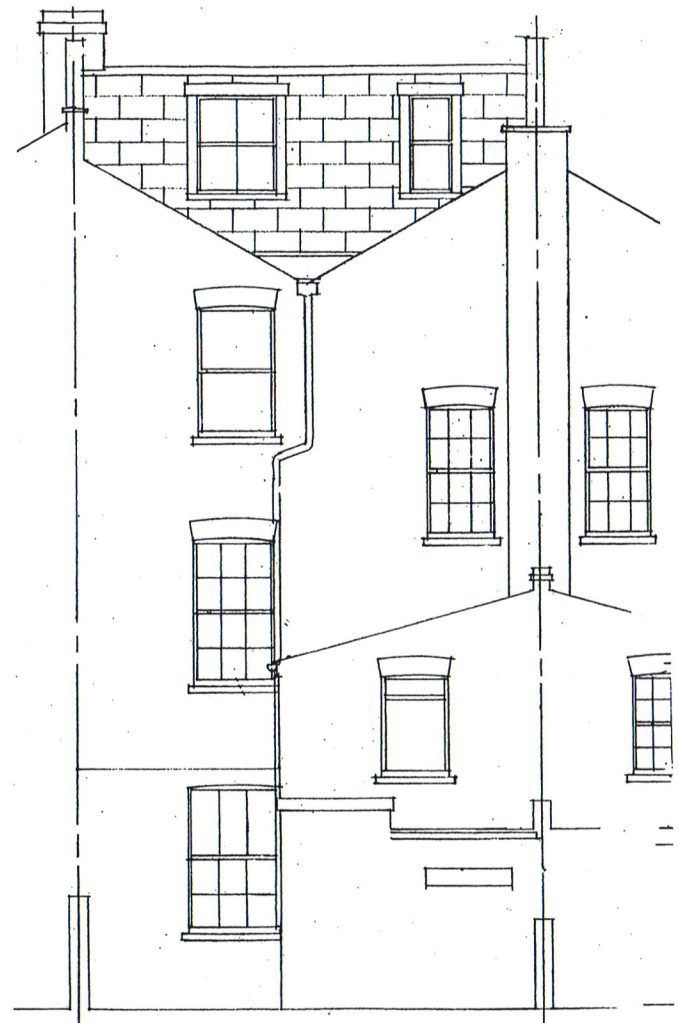
Rear elevation
