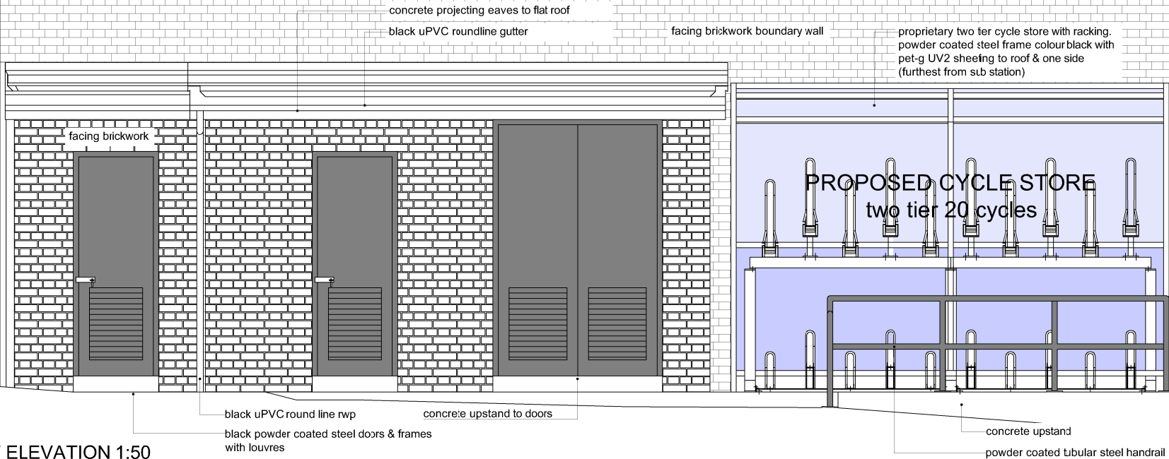
PROPOSED NORTH EAST ELEVATION 1:50 Sub-station & Cycle Store
