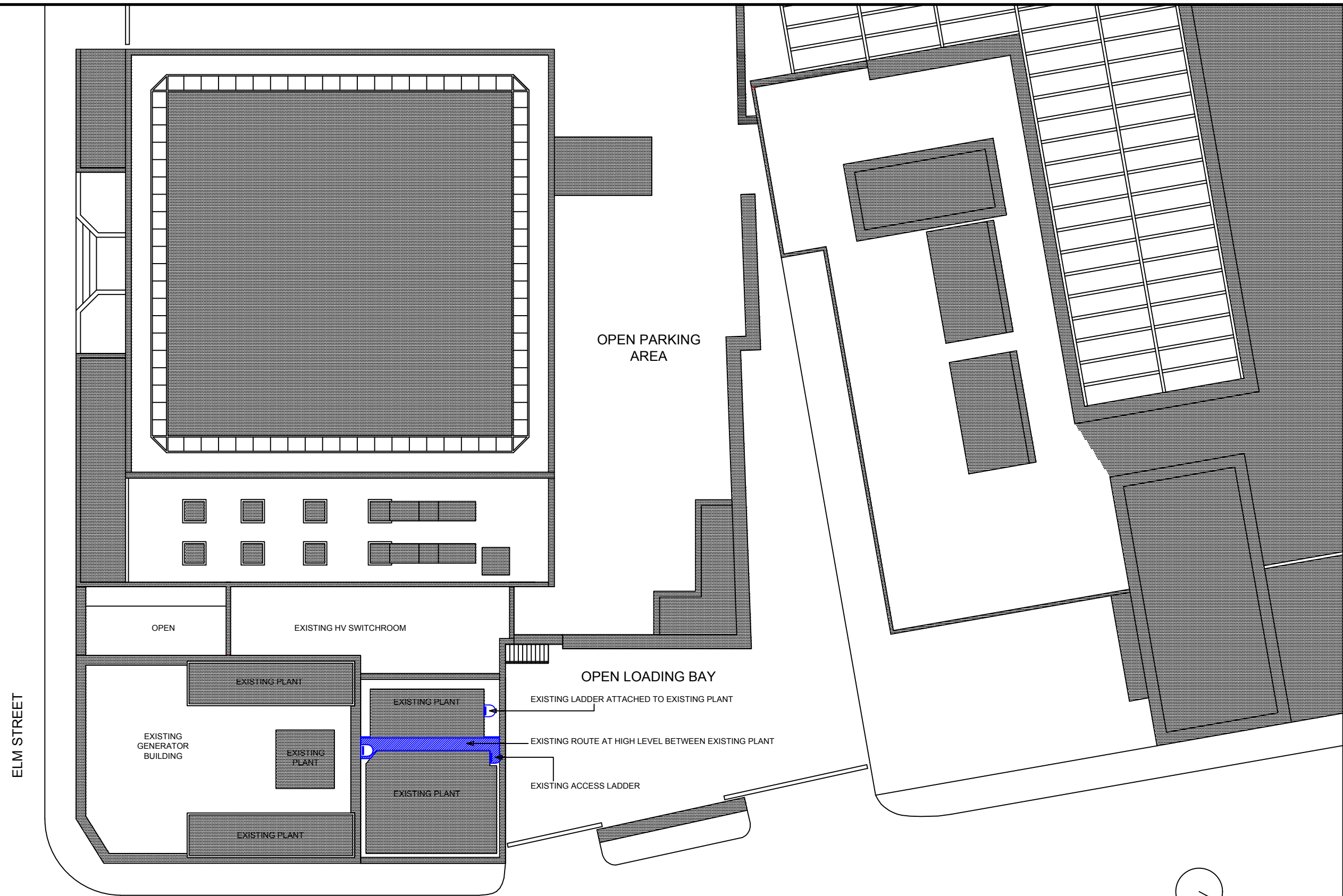
GOUGH STREET ROOF PLAN AS EXISTING SCALE 1:100 AT A1 SCALE 1:200 AT A3
