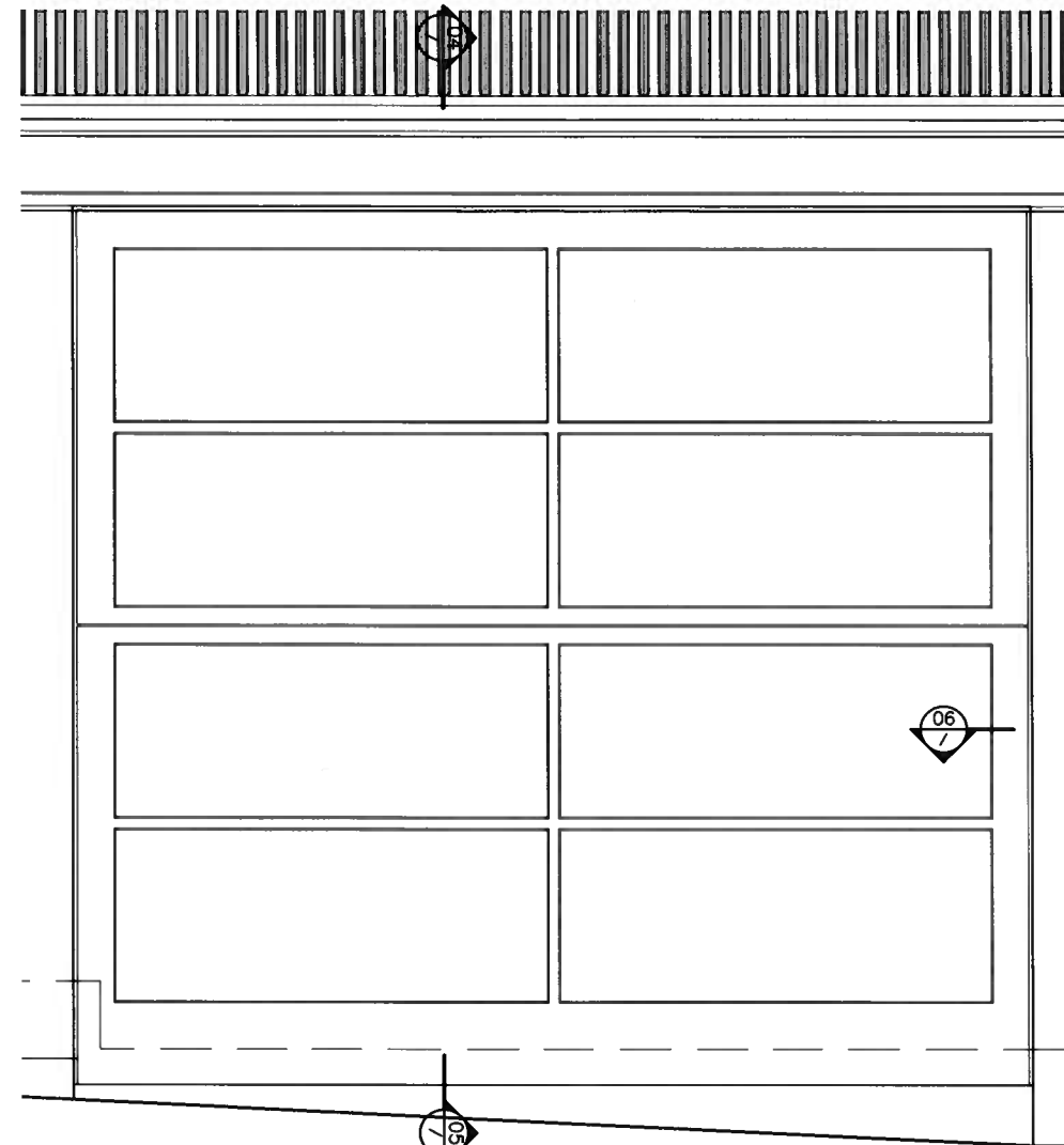
GROUND FLOOR WINDOW ELEVATION SCALE 1:20 @ A3
