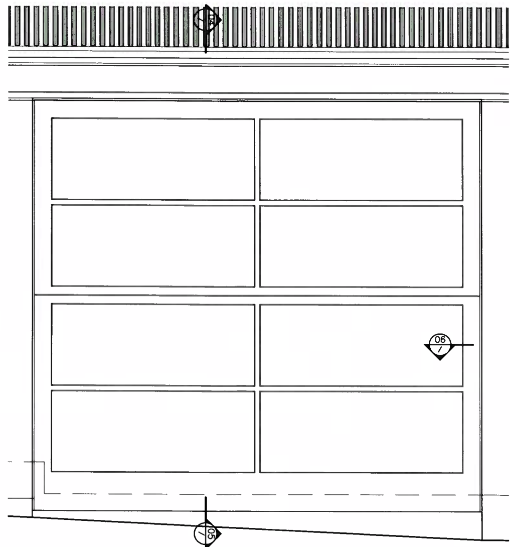
GROUND FLOOR WINDOW ELEVATION SCALE 1:20 @ A3
