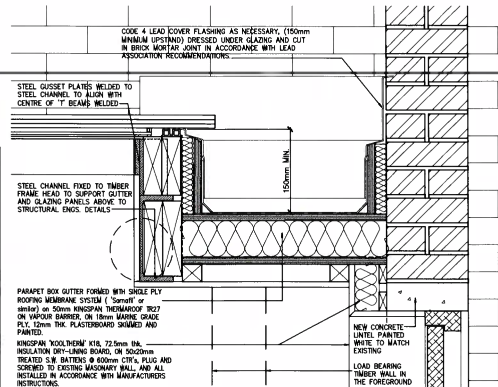
DETAIL OF FIXING NEW GLAZED LINK STRUCTURE TO EXISTING FABRIC
