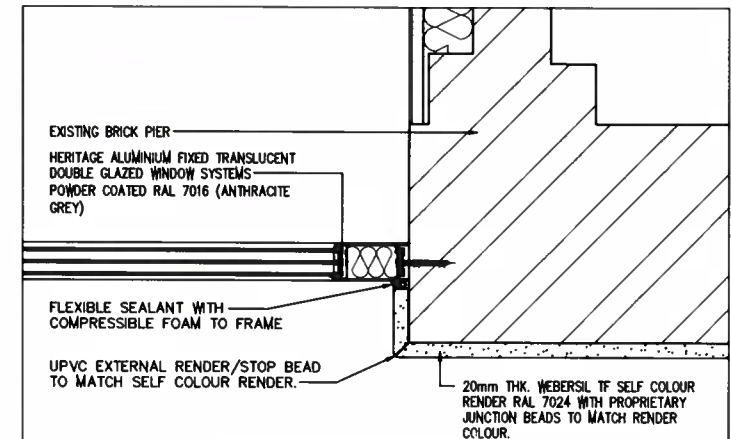
DETAIL 06 - JAMB DETAIL SCALE 1:10 @ A3
