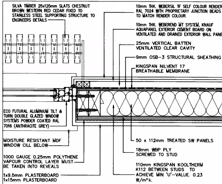
DETAIL 03 - JAMB DETAIL SCALE 1:10 @ A3
