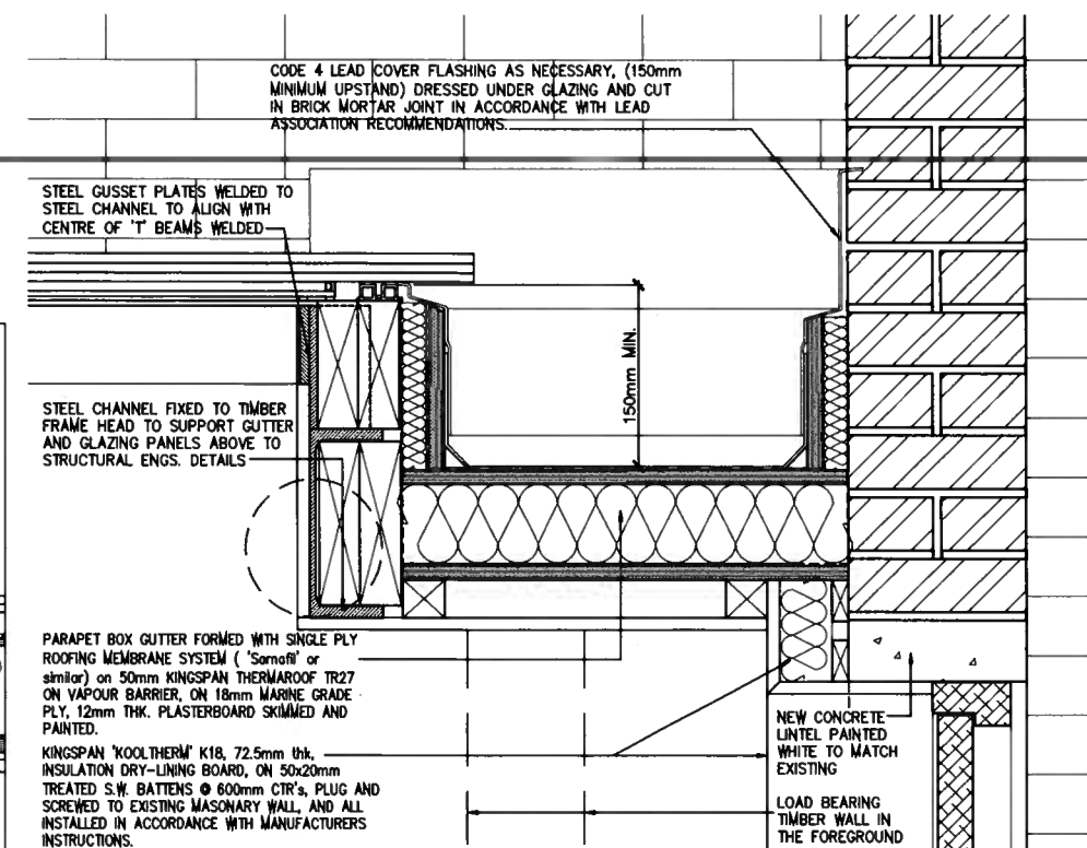
DETAIL OF FIXING NEW GLAZED LINK STRUCTURE TO EXISTING FABRIC SCALE 1:10 @ A3
