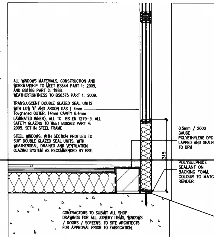
DETAIL 05 - CILL DETAIL SCALE 1:10 @ A3
