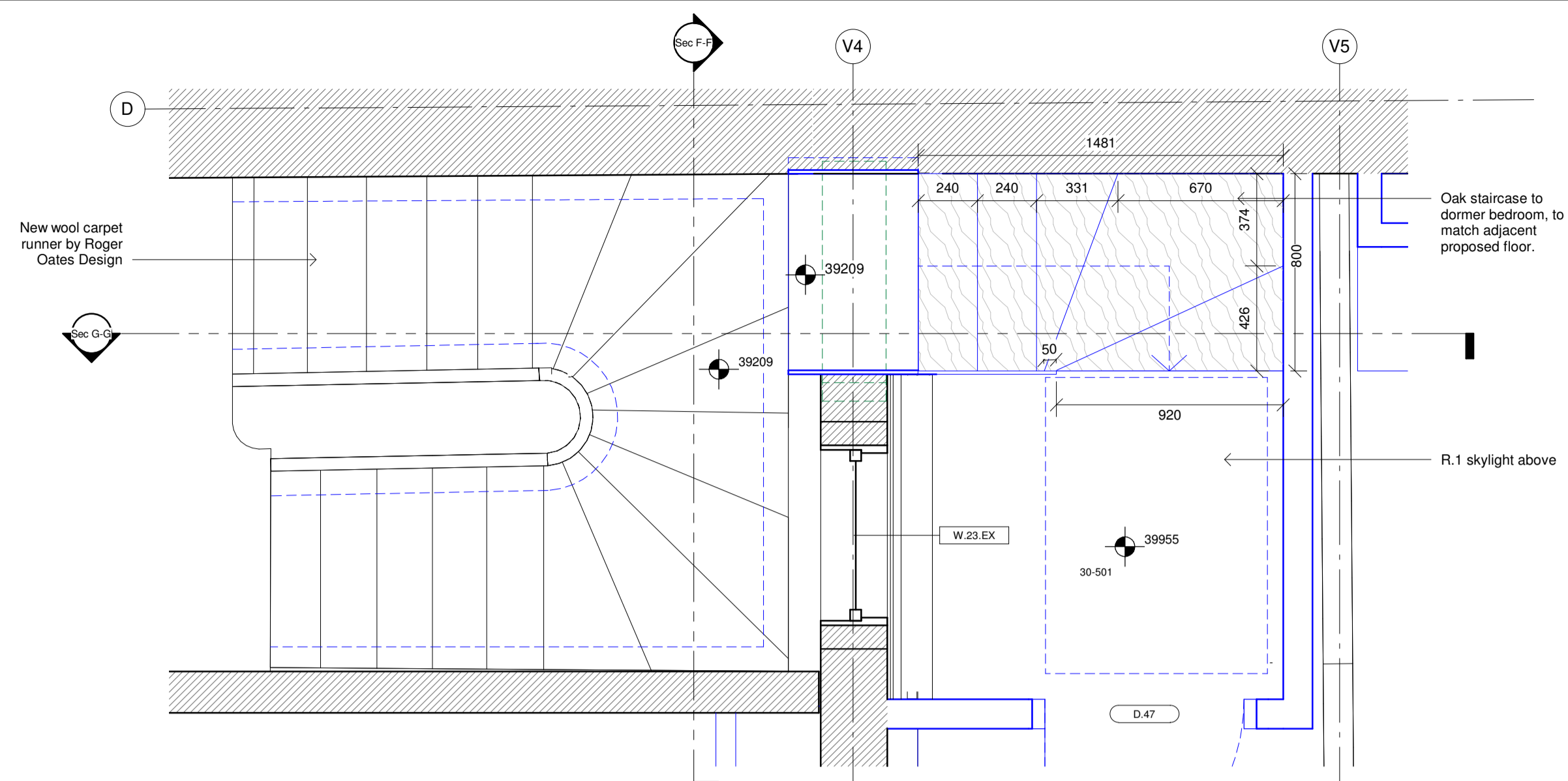
Vicarage - First Floor Plan 1:20
