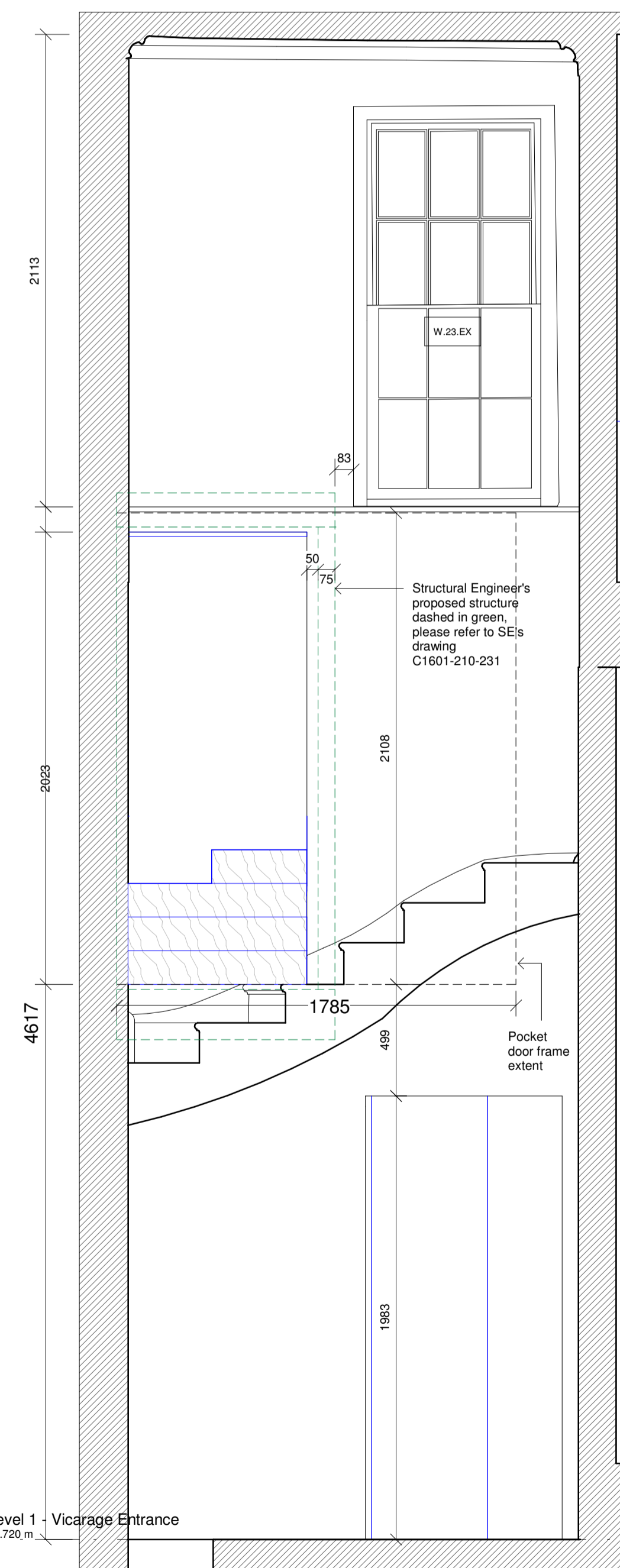
Vicarage - Cross-Section B_B - Proposed 1:20
