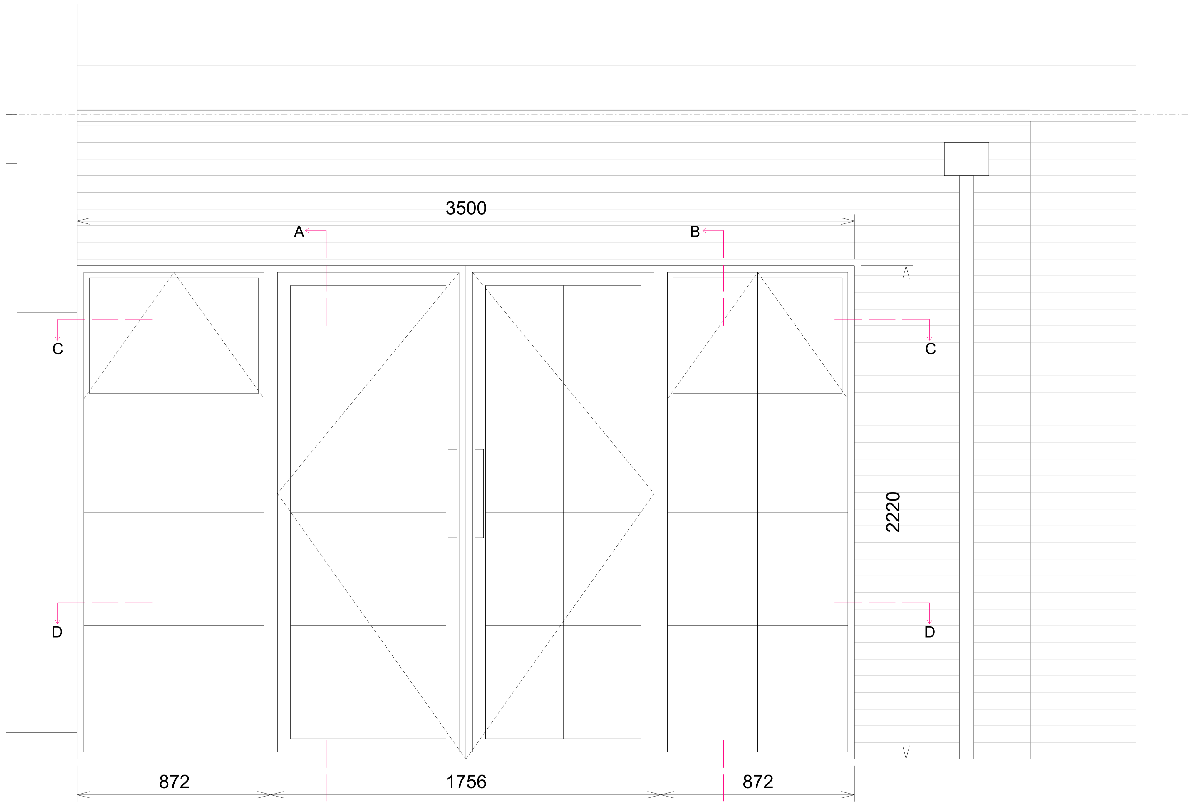
Elevation 1:10
