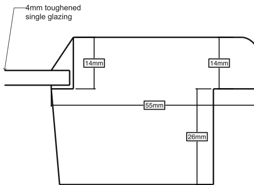
Section E-E
