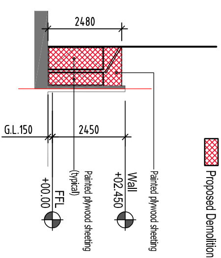
Existing Side Passage (Part) Front Elevation (West)
