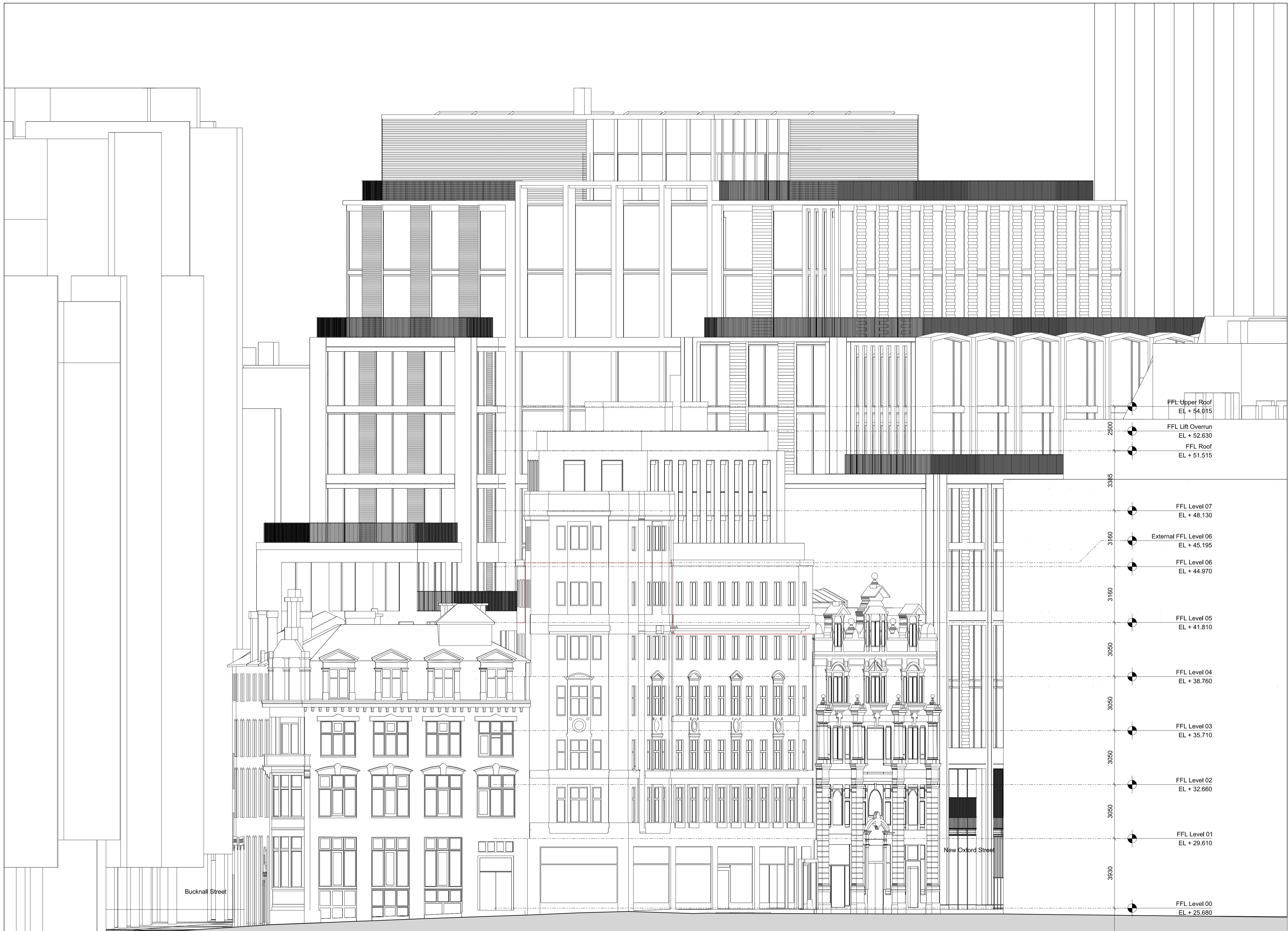
01 Medius House East Elevation 1:100
