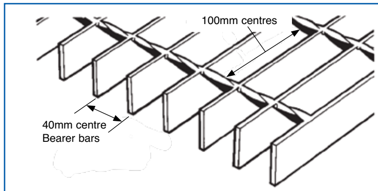
TYPE W100 - 40 / 100
