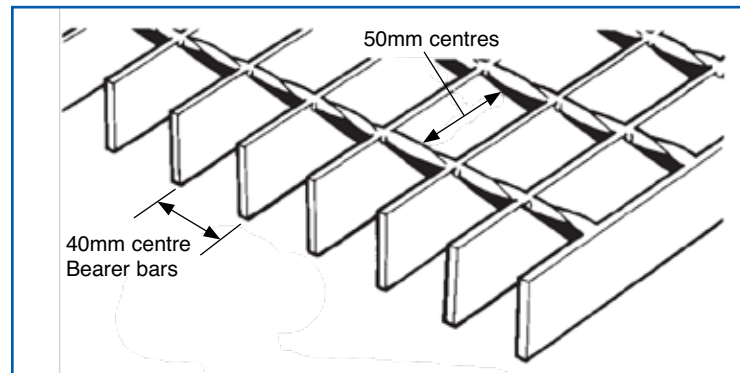
TYPE W50 - 40 / 50
