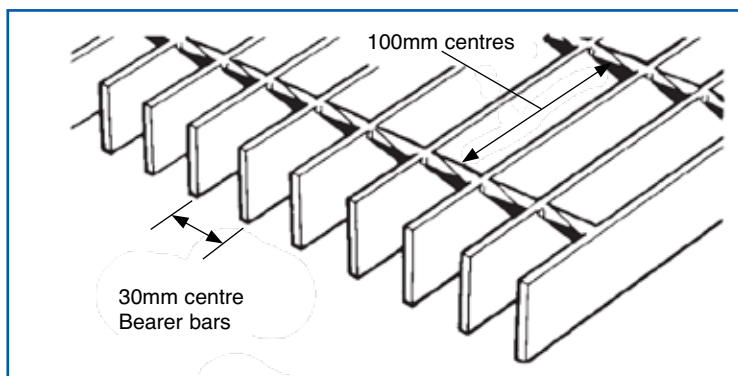
TYPE N100 - 30 / 100
