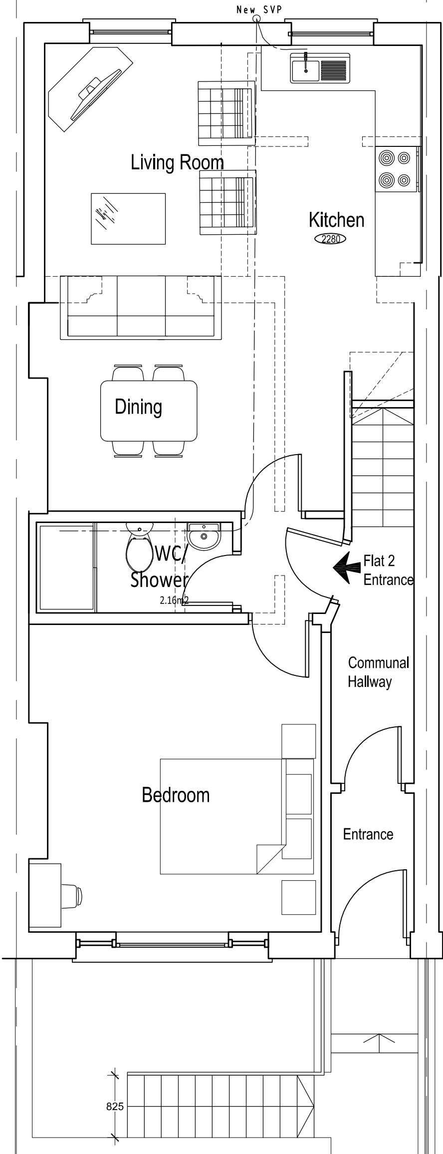
7A PROPOSED GROUND FLOOR PLAN SCALE 1:50
