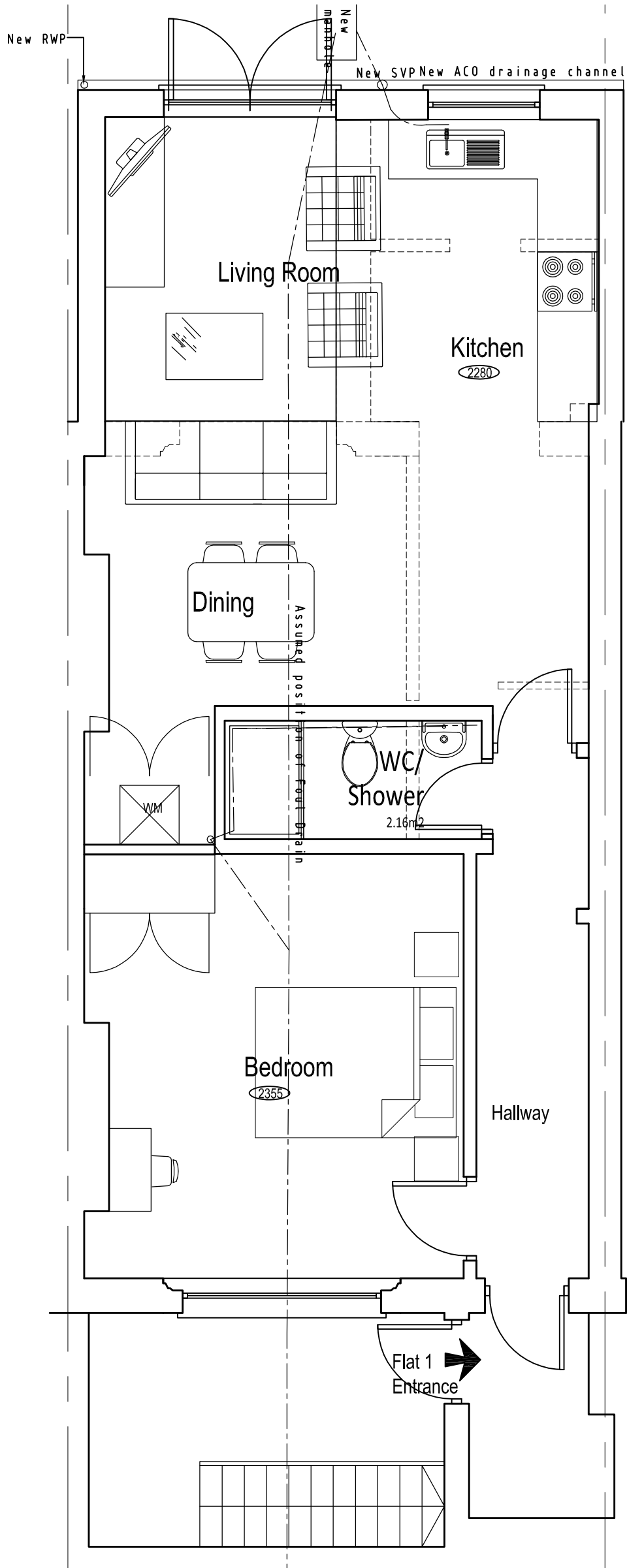
7A PROPOSED LOWER GROUND FLOOR PLAN SCALE 1:50
