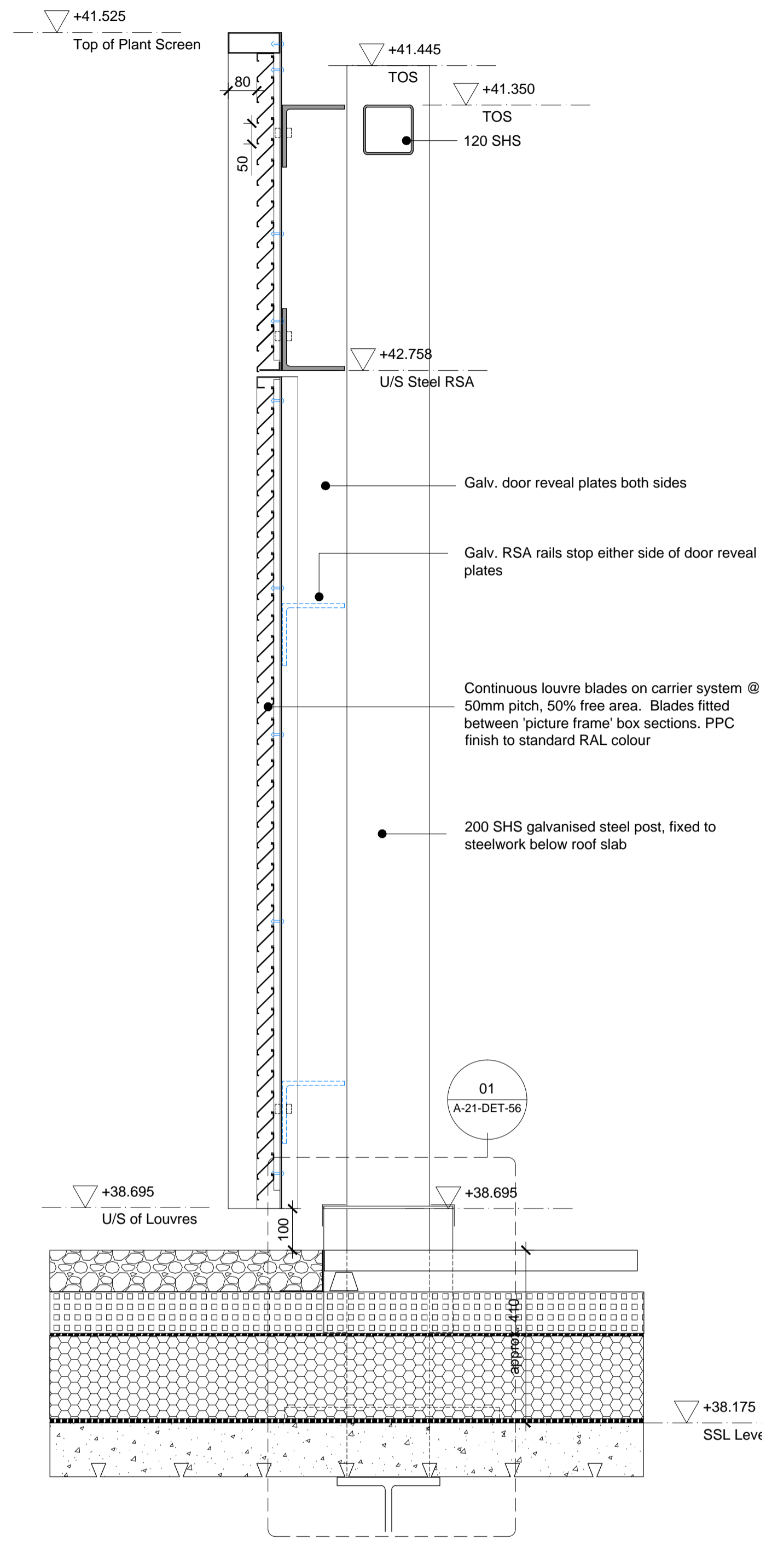
02 Charterhouse St. Plant Screen - Typ Section at Louvred Door A-21-DET-55 SCALE: 1:10
