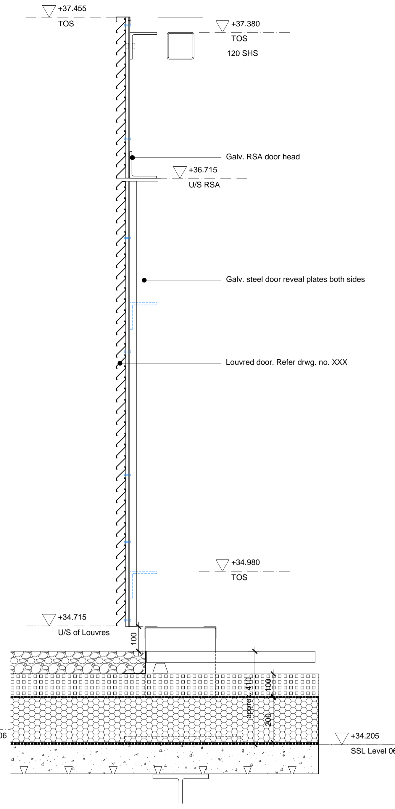
02 Saffron Hill Plant Screen - Typ Section at Louvred Door A-21-DET-54 SCALE: 1:10
