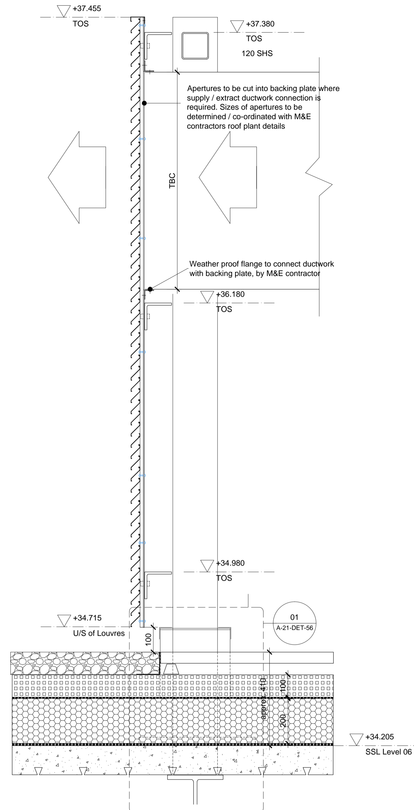
03 Saffron Hill Plant Screen - Typ Section Ductwork Connection A-21-DET-54 SCALE: 1:10
