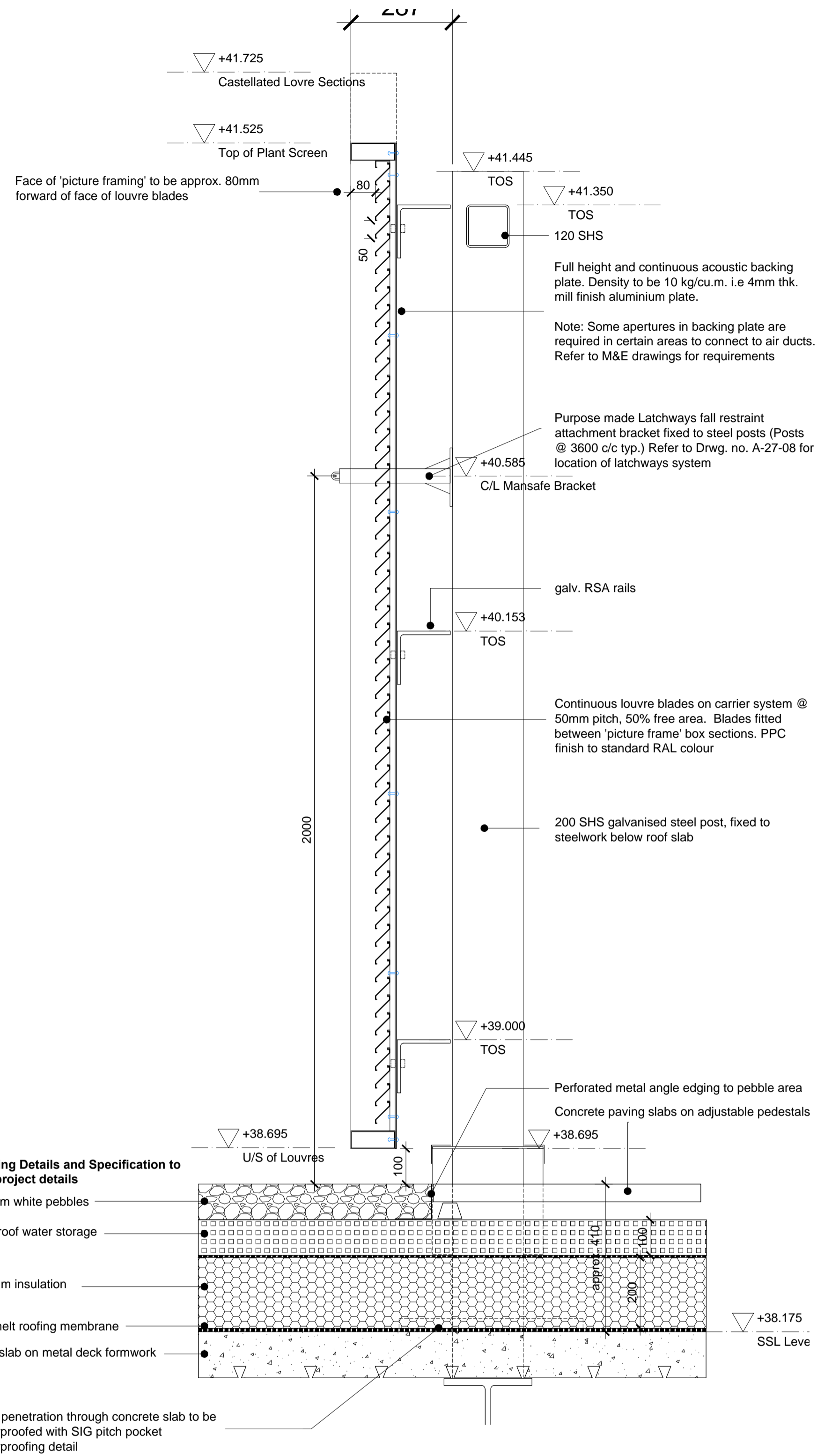
01 Charterhouse St. Plant Screen - Typ Section A-21-DET-55 SCALE: 1:10
