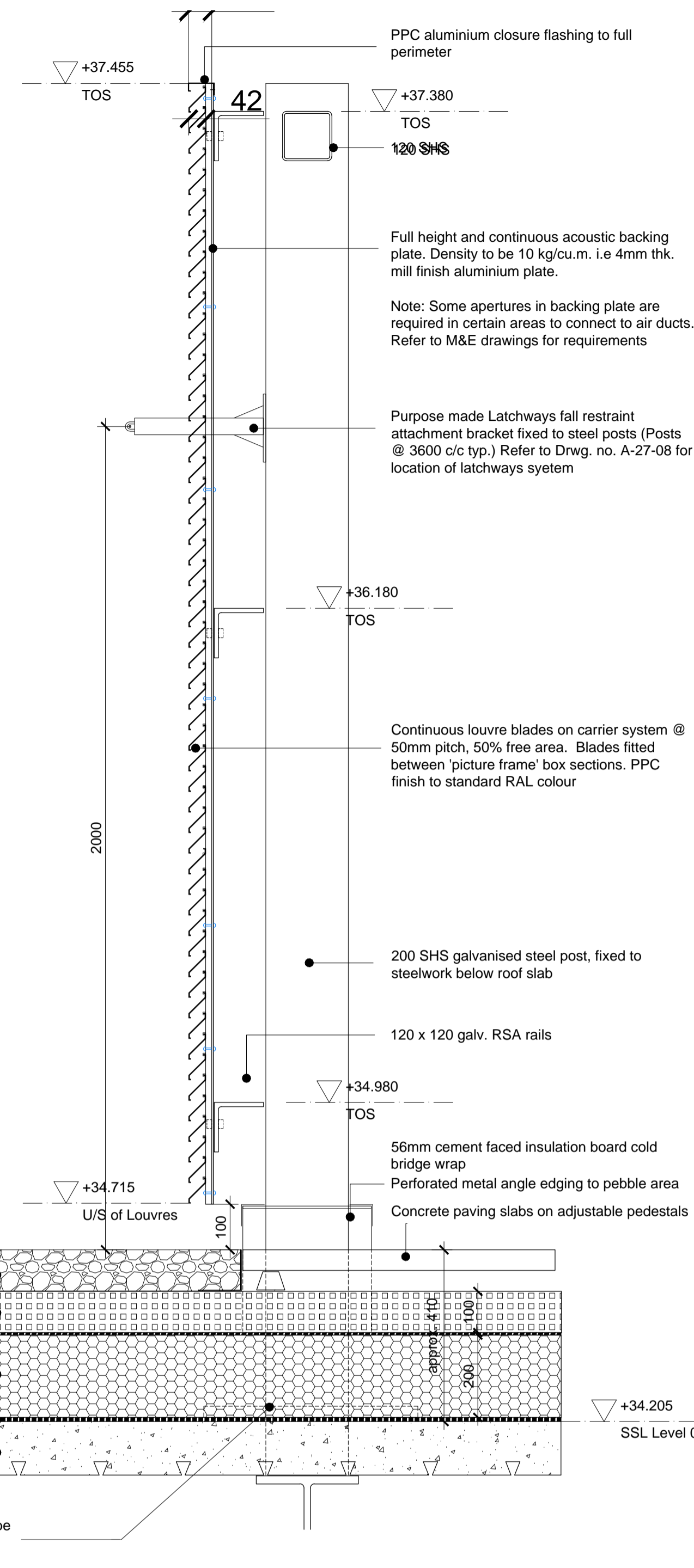
01 Saffron Hill Plant Screen - Typ Section A-21-DET-54 SCALE: 1:10
