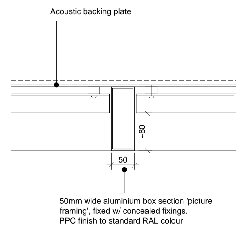
05 Charterhouse St. Plant Screen - Typ. Frame Detail A-21-DET-56 SCALE: 1:5
