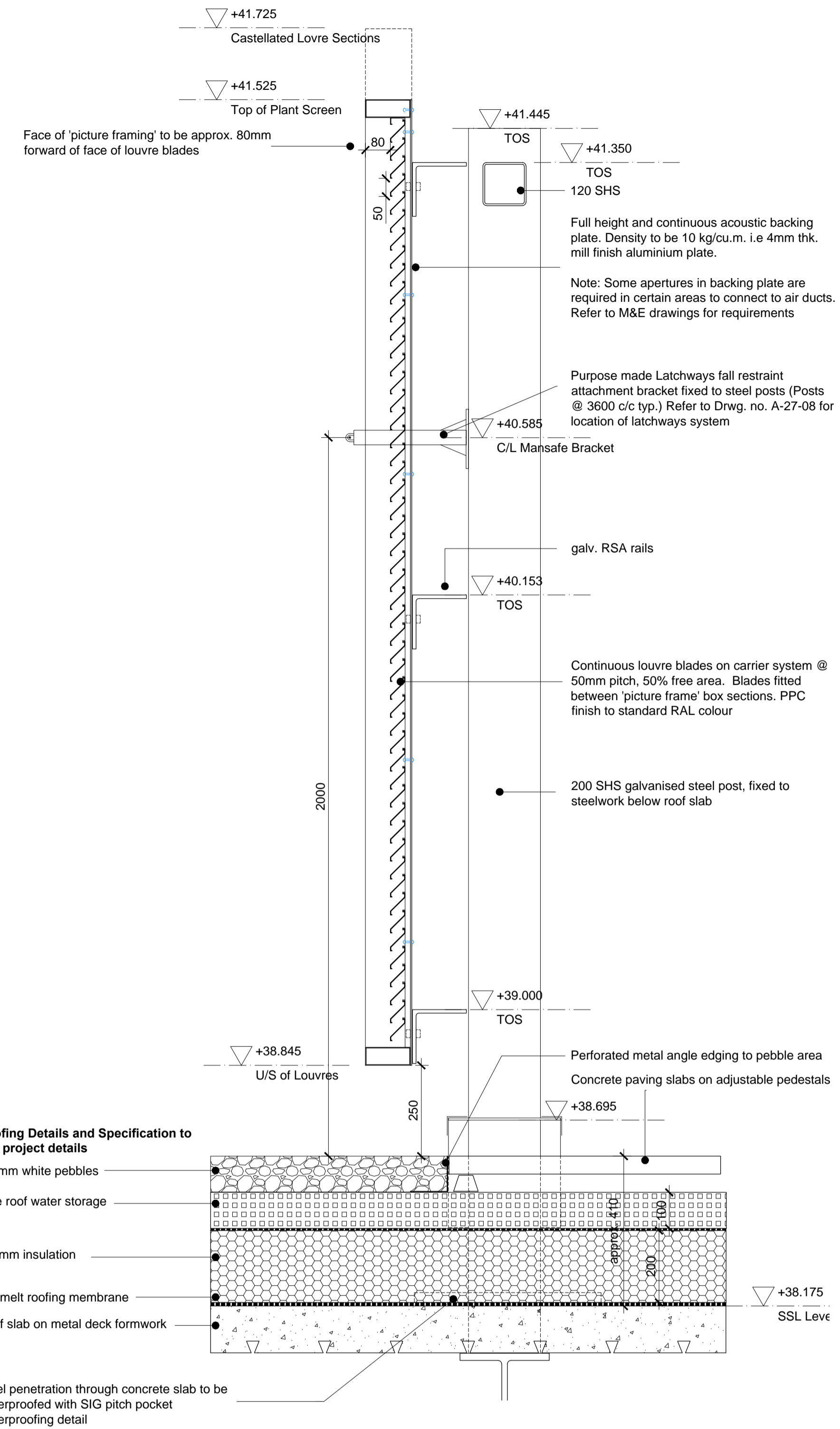
03 Charterhouse St. Plant Screen - Undercut Section Section A-21-DET-55 SCALE: 1:10
