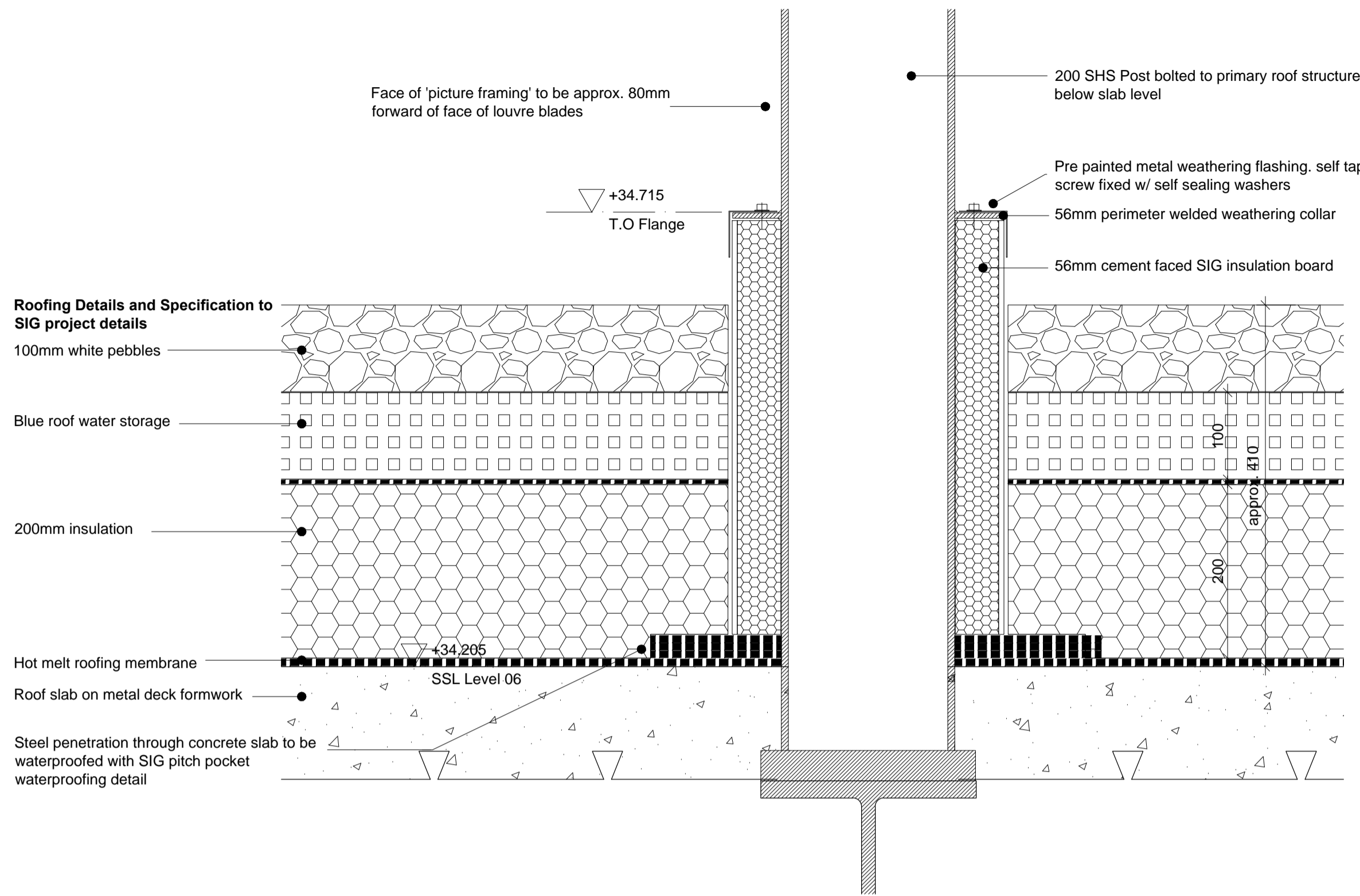
01 Plant Screen - Steel Post Base Details A-21-DET-56 SCALE: 1:5
