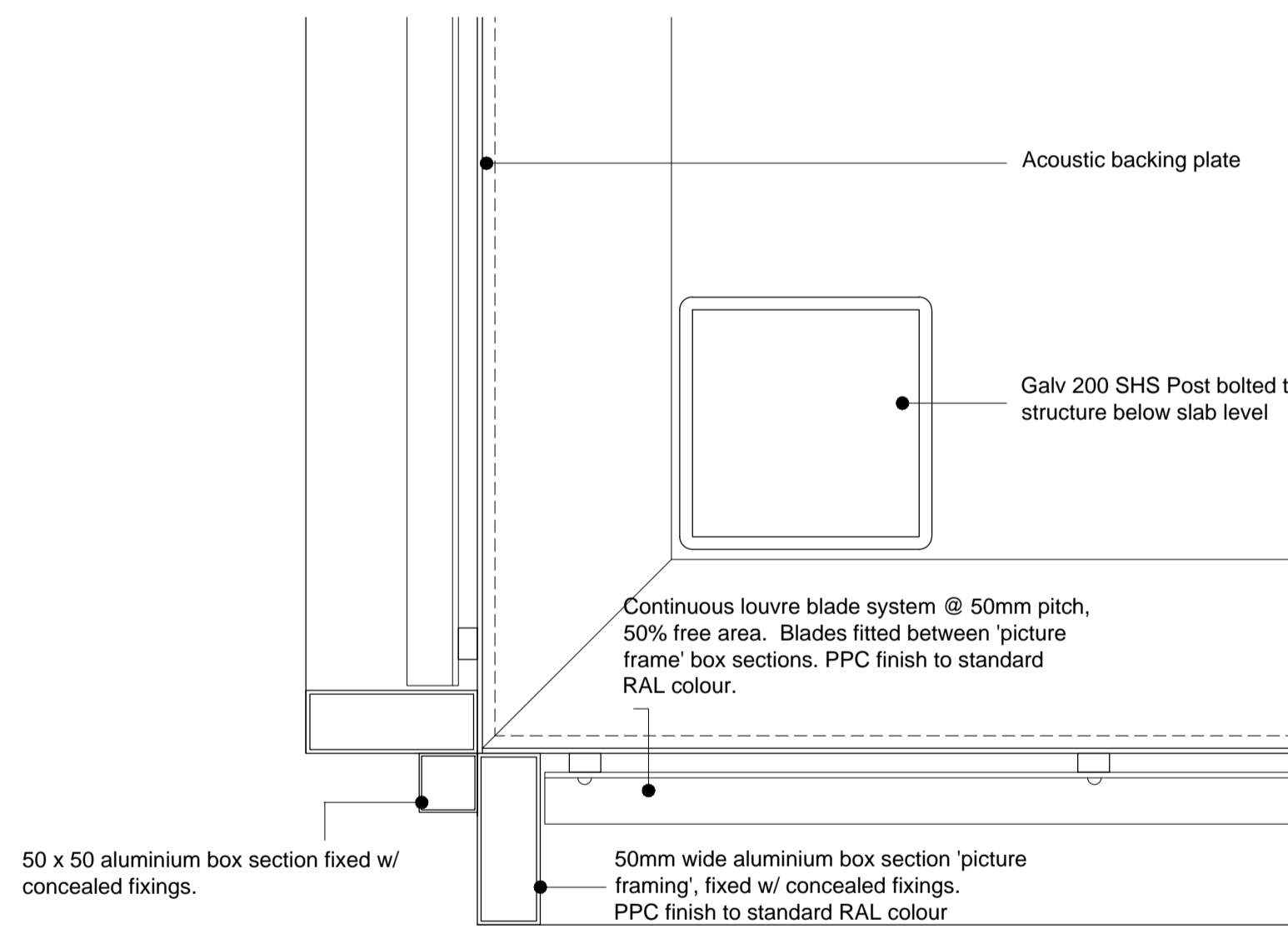
01 Plant Screen - Steel Post Base Details A-21-DET-56 SCALE: 1:5
