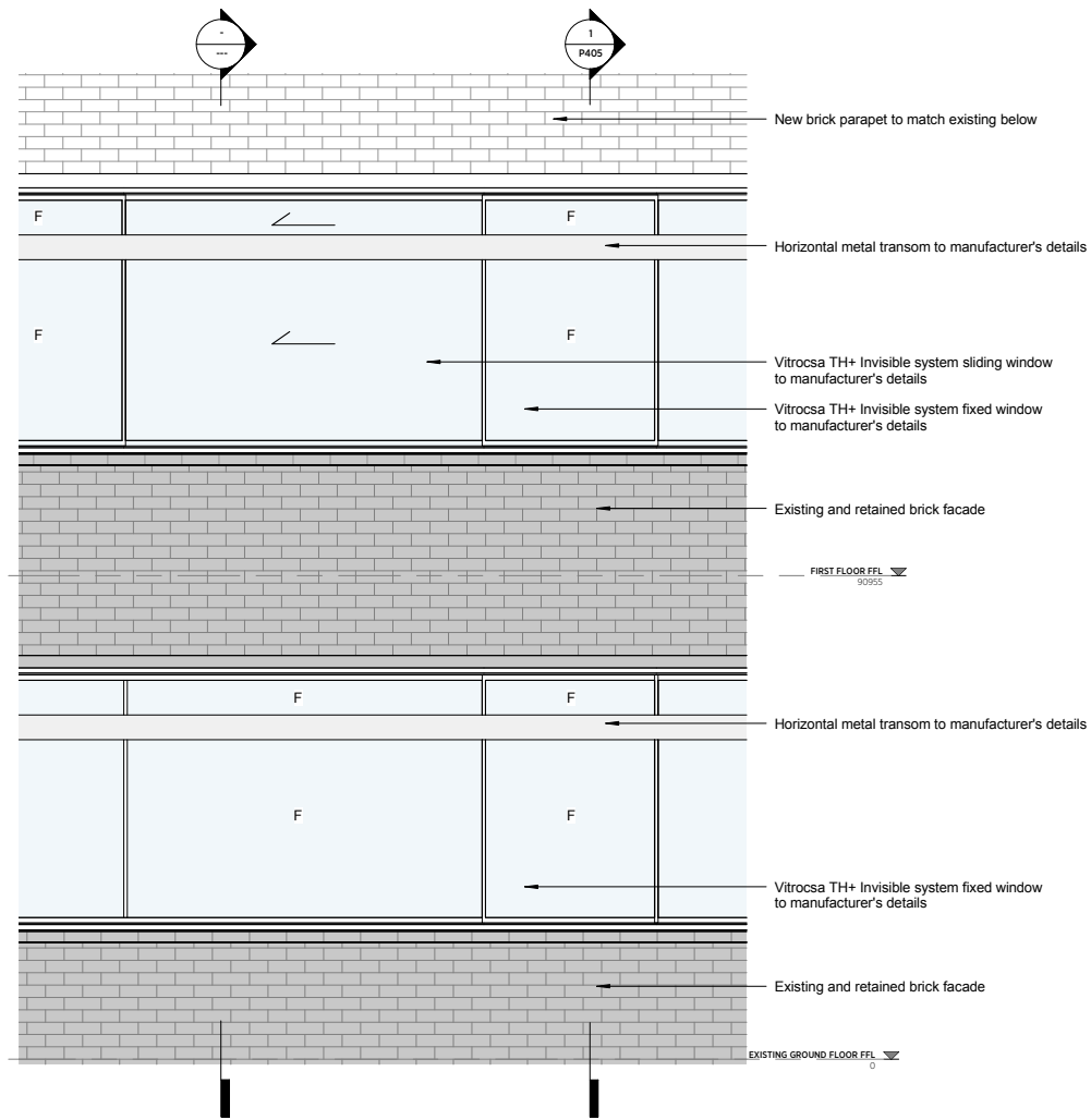
2 EXTRACT OF FRONT FACADE WINDOW ELEVATION 1:25
