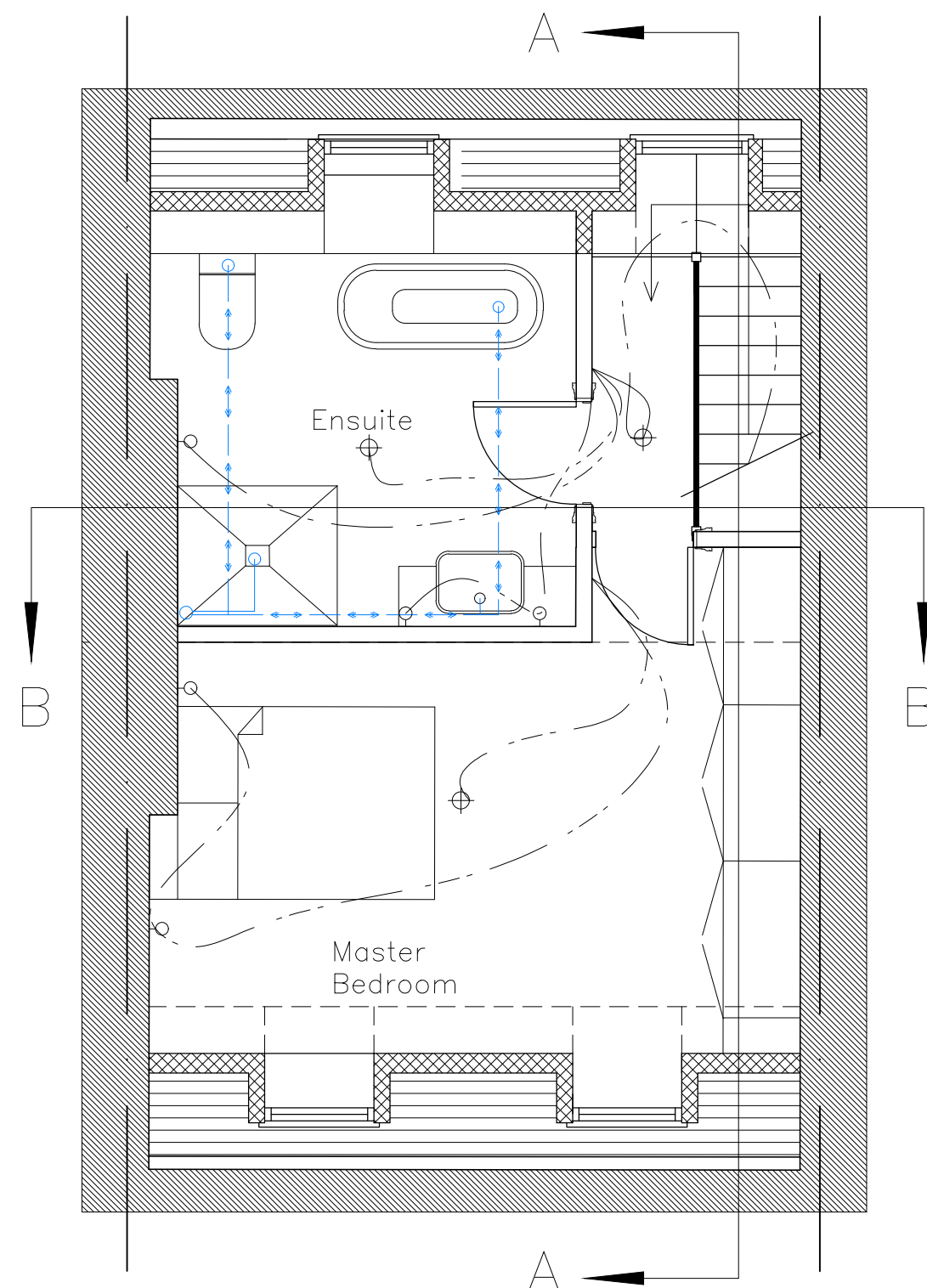
Proposed Third Floor
