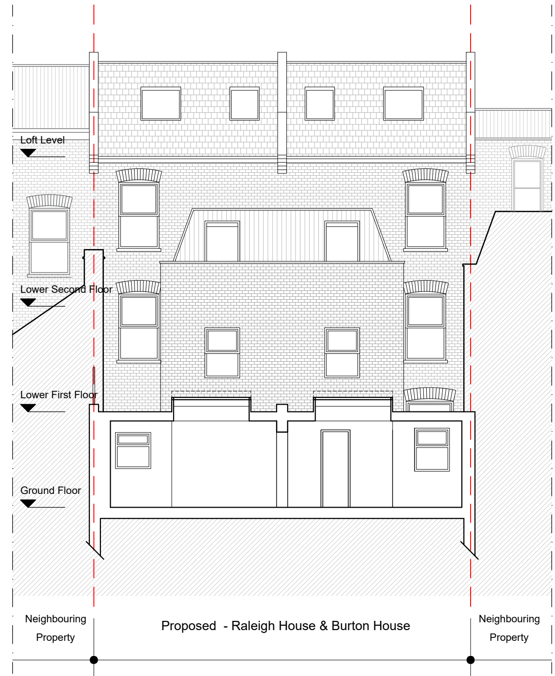
Rear Elevation
