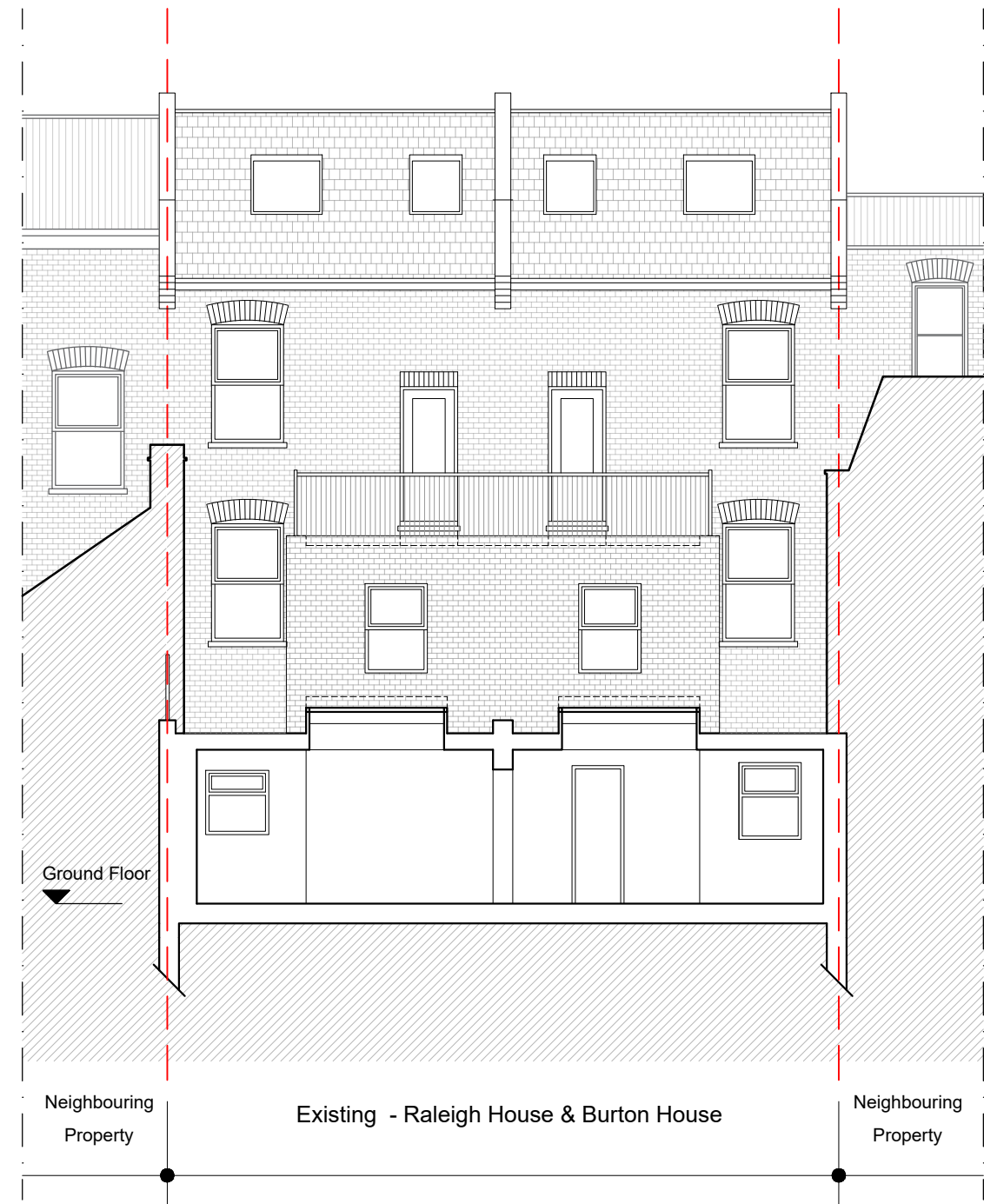
Rear Elevation
