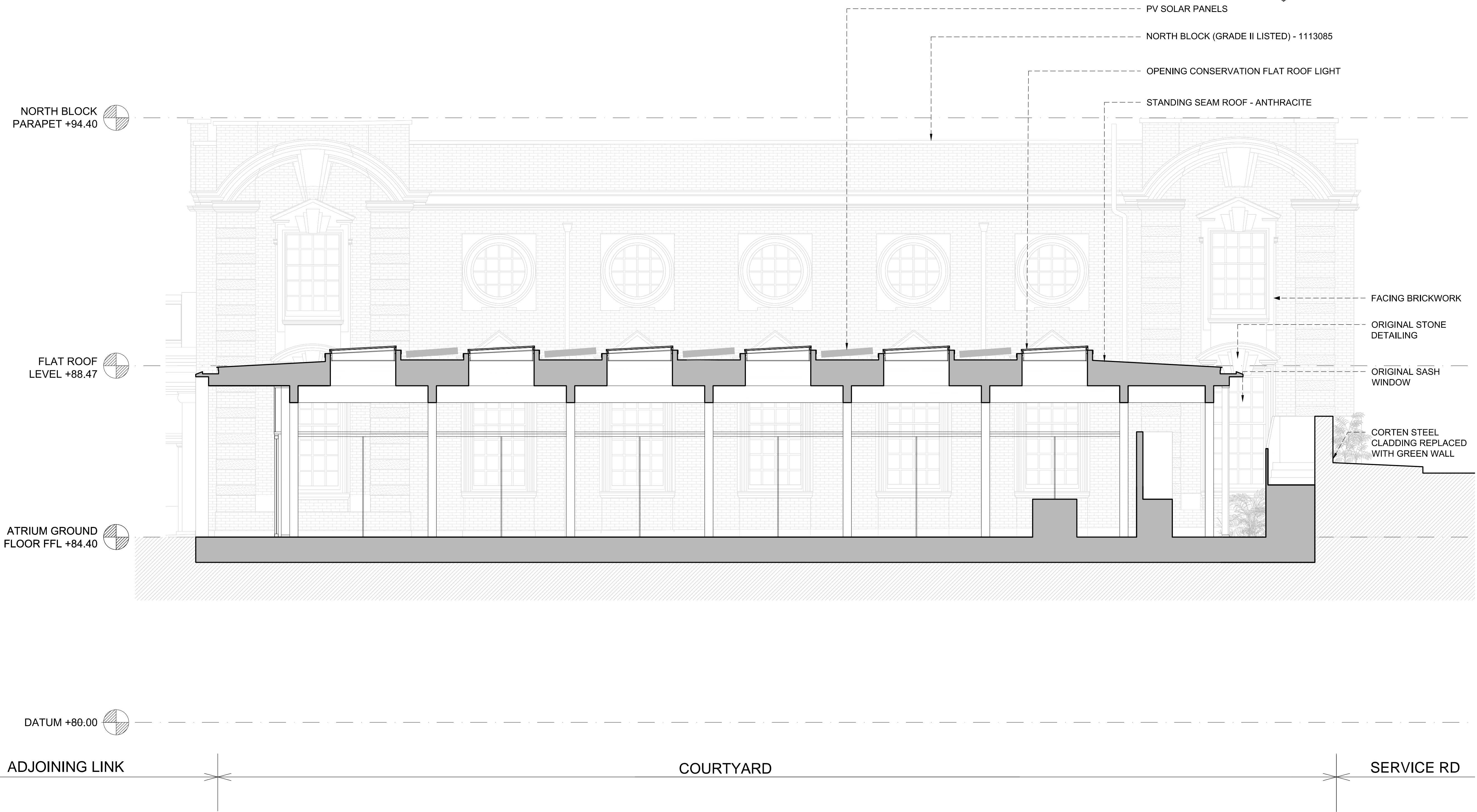
PROPOSED SECTION A @ 1:50 (A1)
