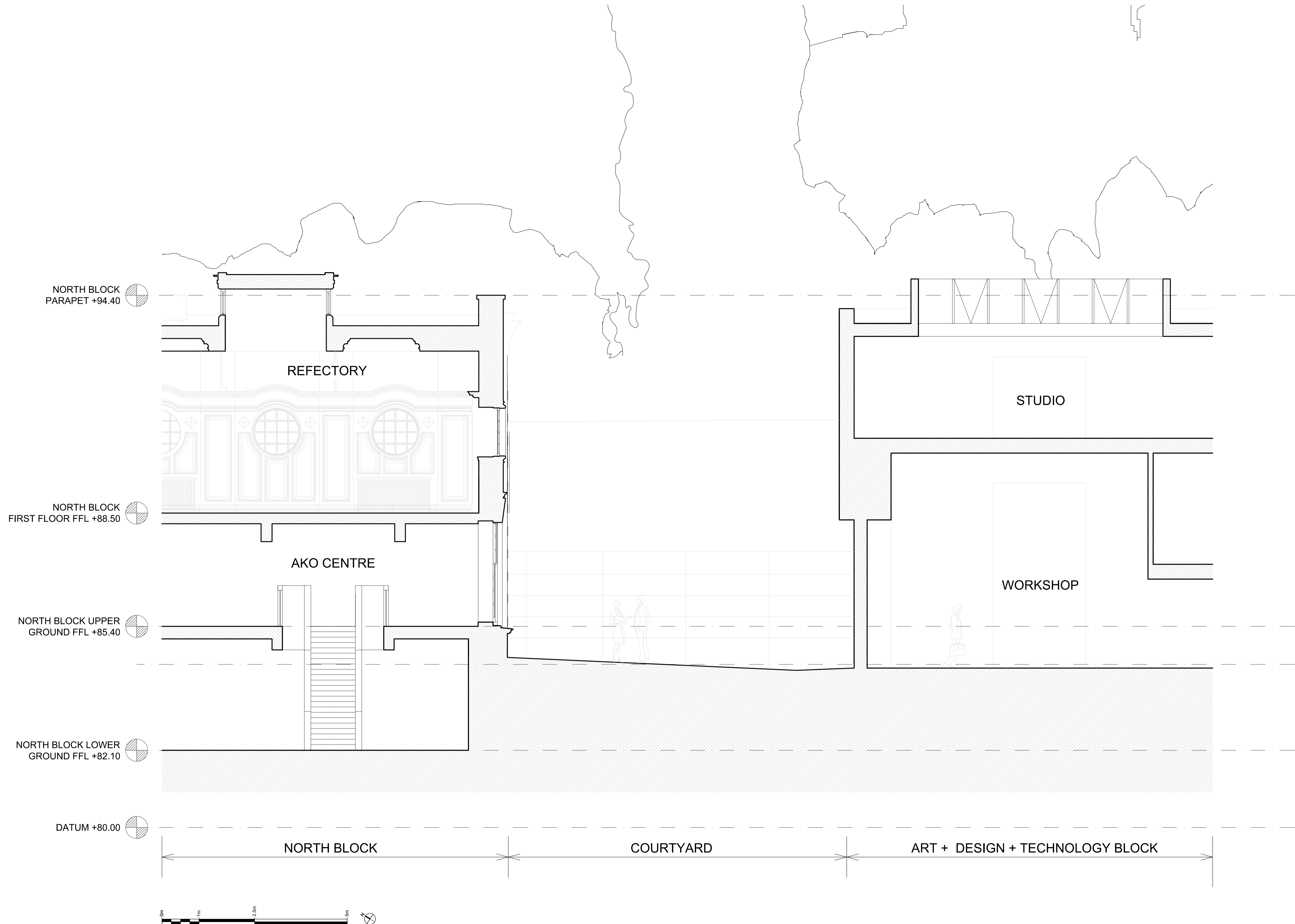
PROPOSED SECTION B @ 1:50 (A1)
