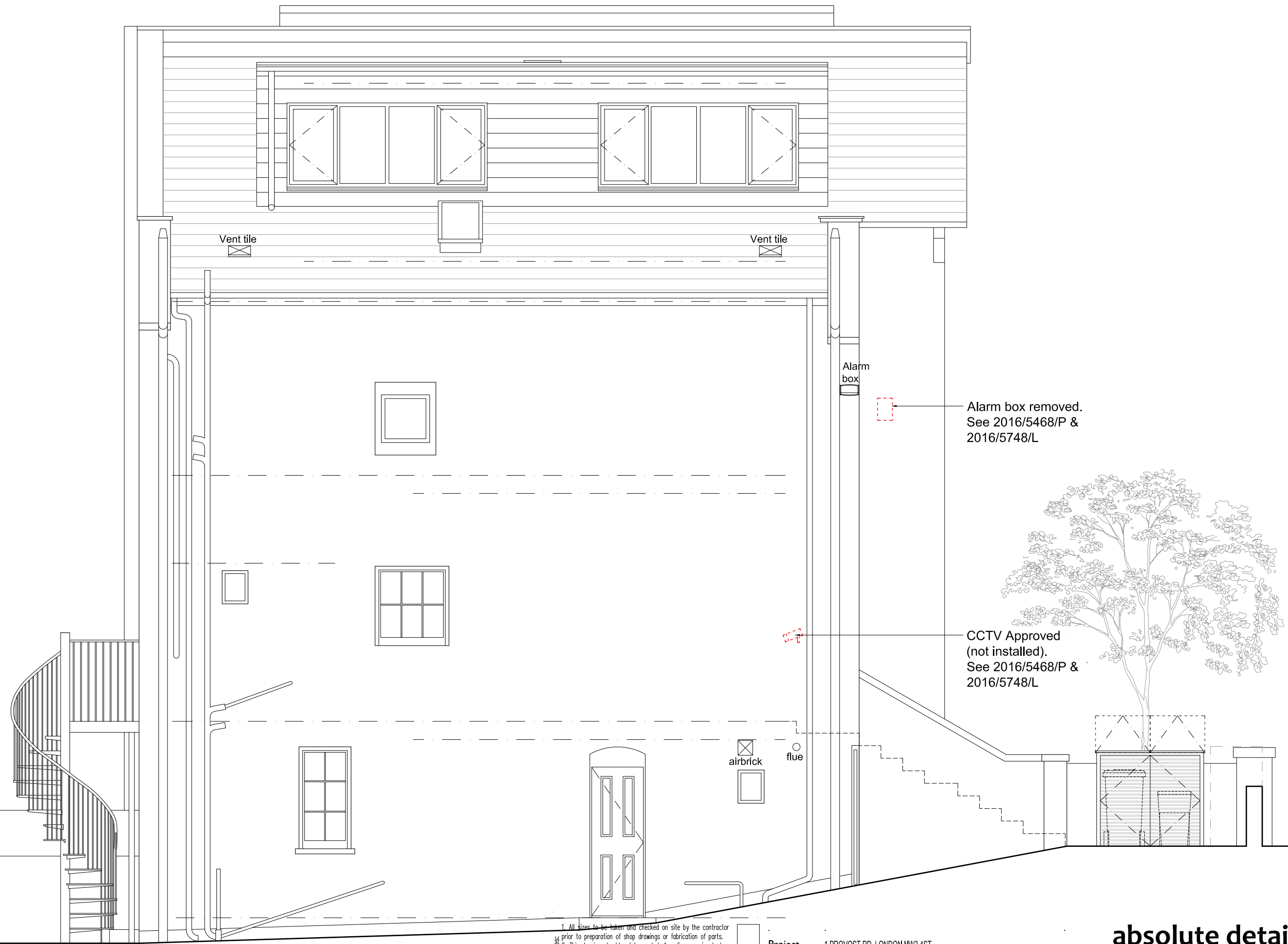
Flank (side) Elevation as Existing
