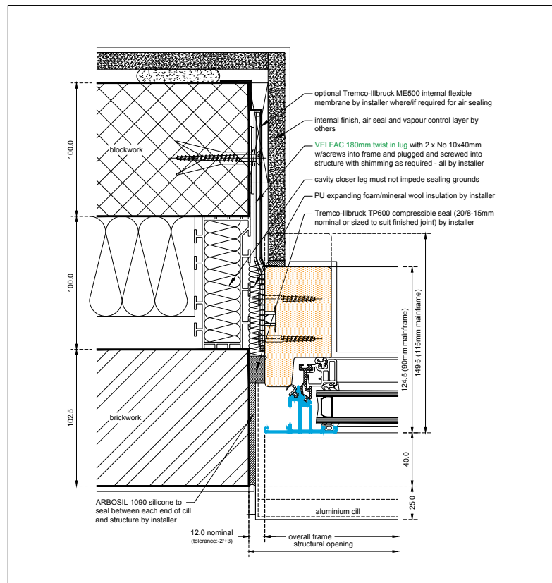
01 PROPOSED WINDOW JAMB DETAIL SCALE 1:2
