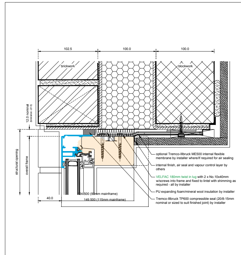
02 PROPOSED WINDOW HEAD DETAIL SCALE 1:2
