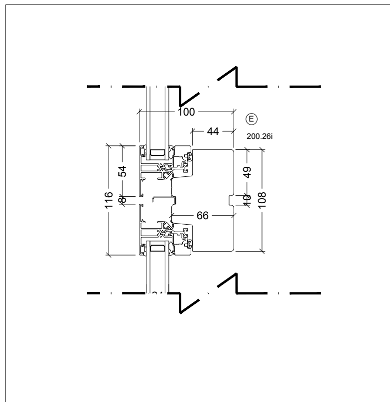
04 PROPOSED WINDOW SECTION DETAIL SCALE 1:2
