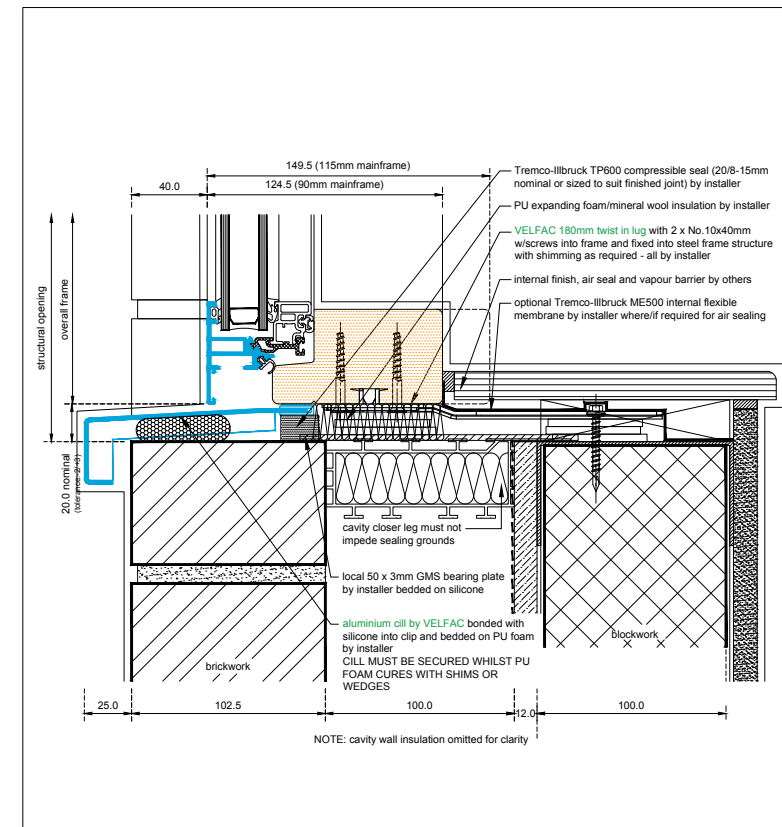
03 PROPOSED WINDOW SILL DETAIL SCALE 1:2
