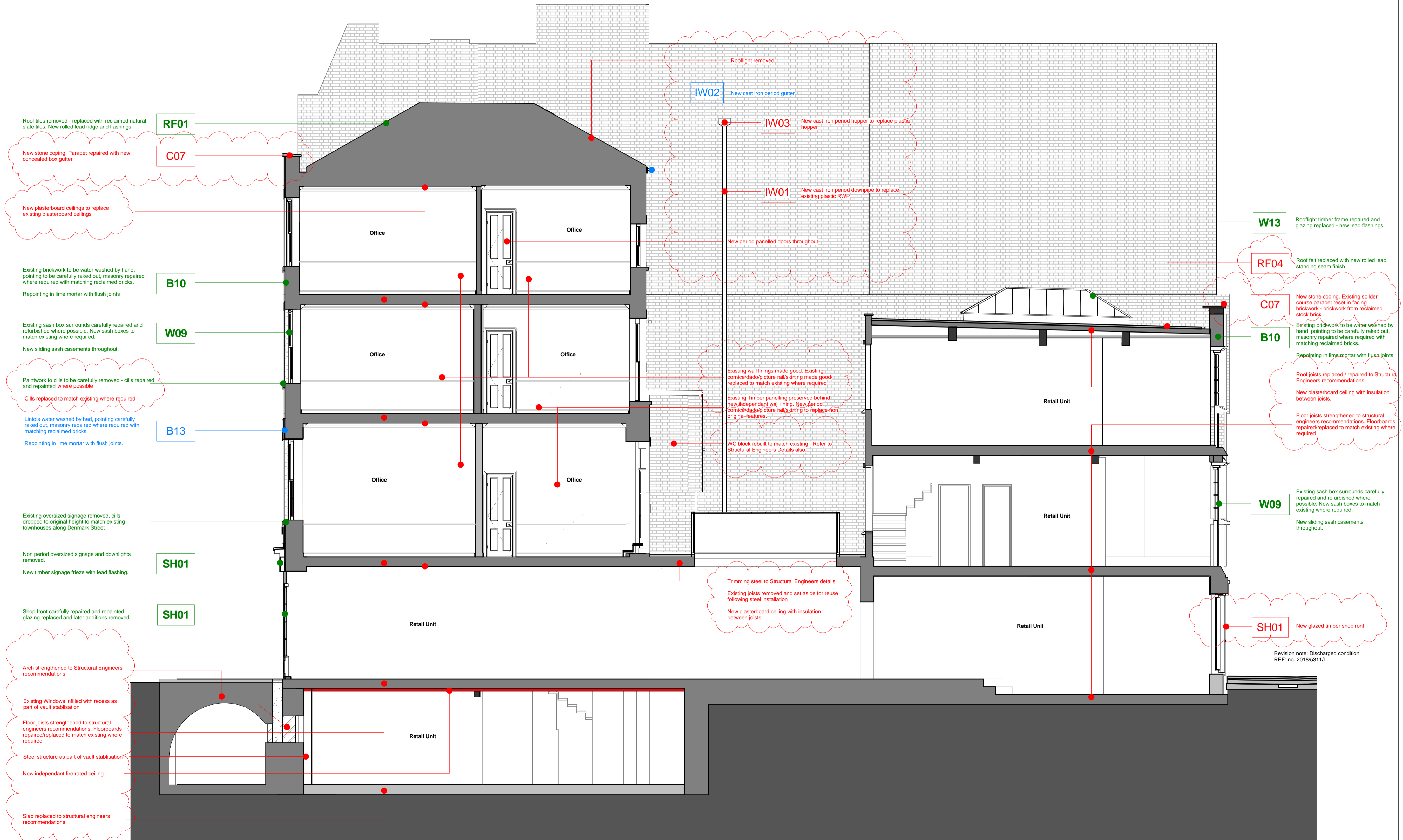
1 No. 20 Denmark Street Detail Section. Scale: 1 : 50
