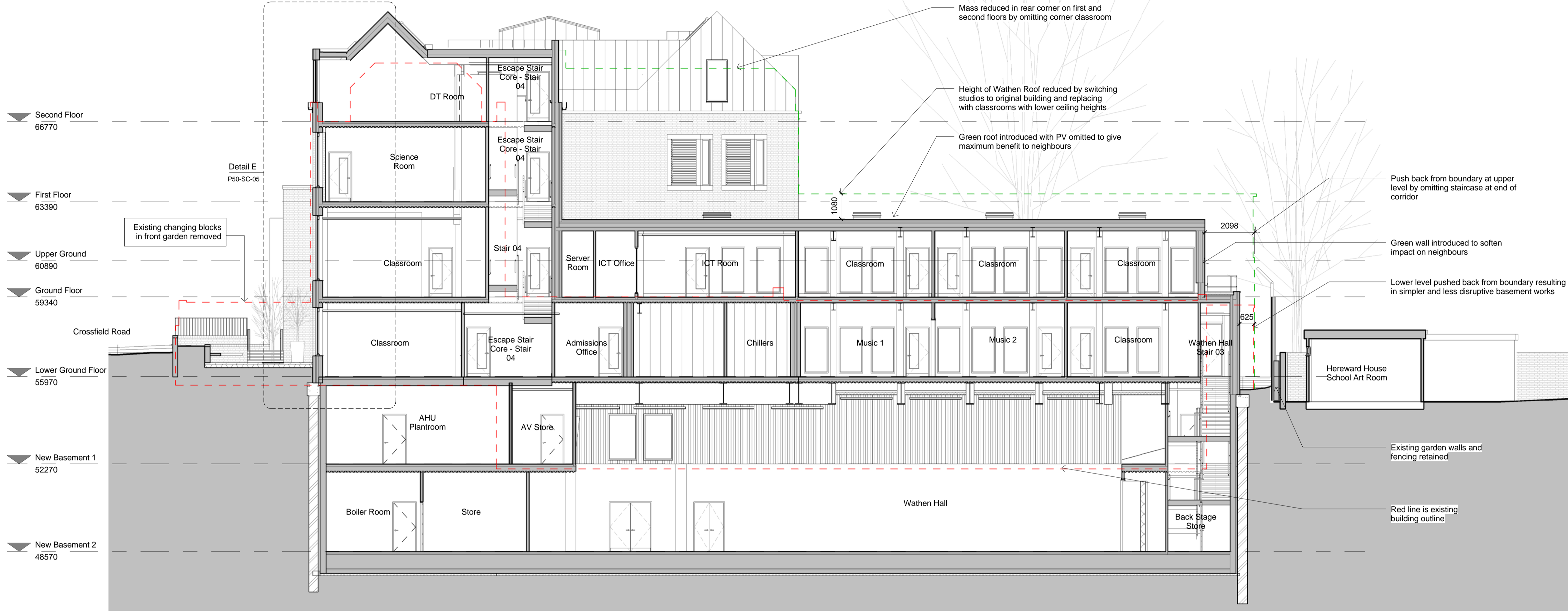
Proposed Section B 1 : 100
