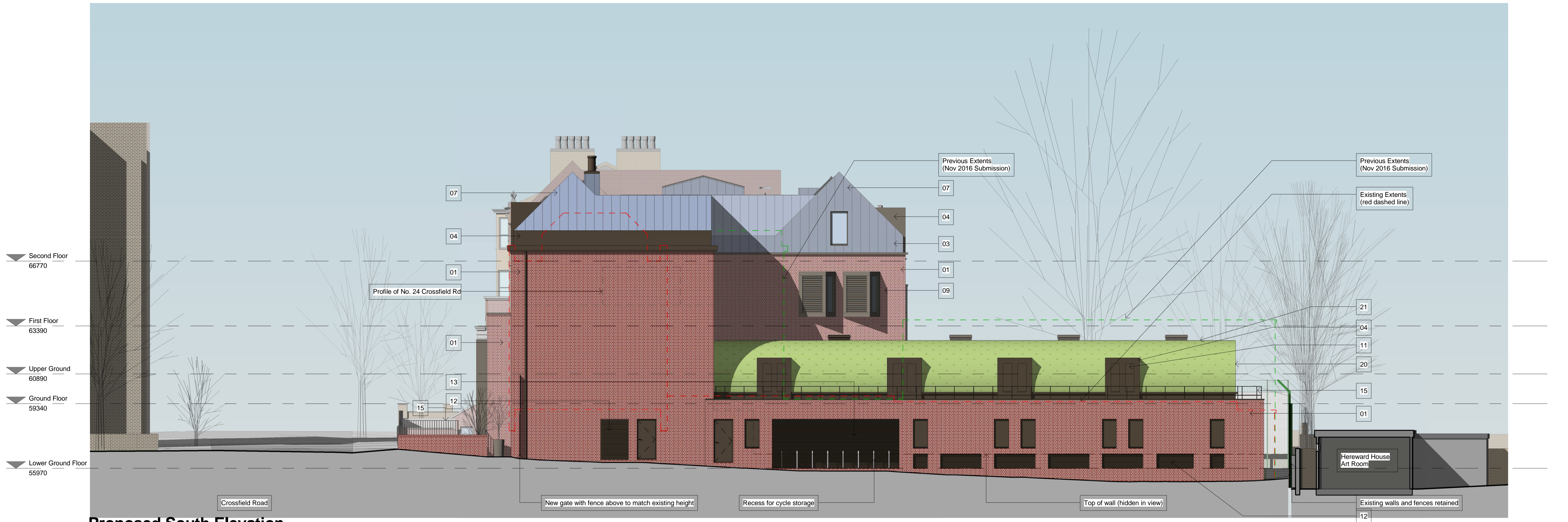
Proposed South Elevation 1 : 100
