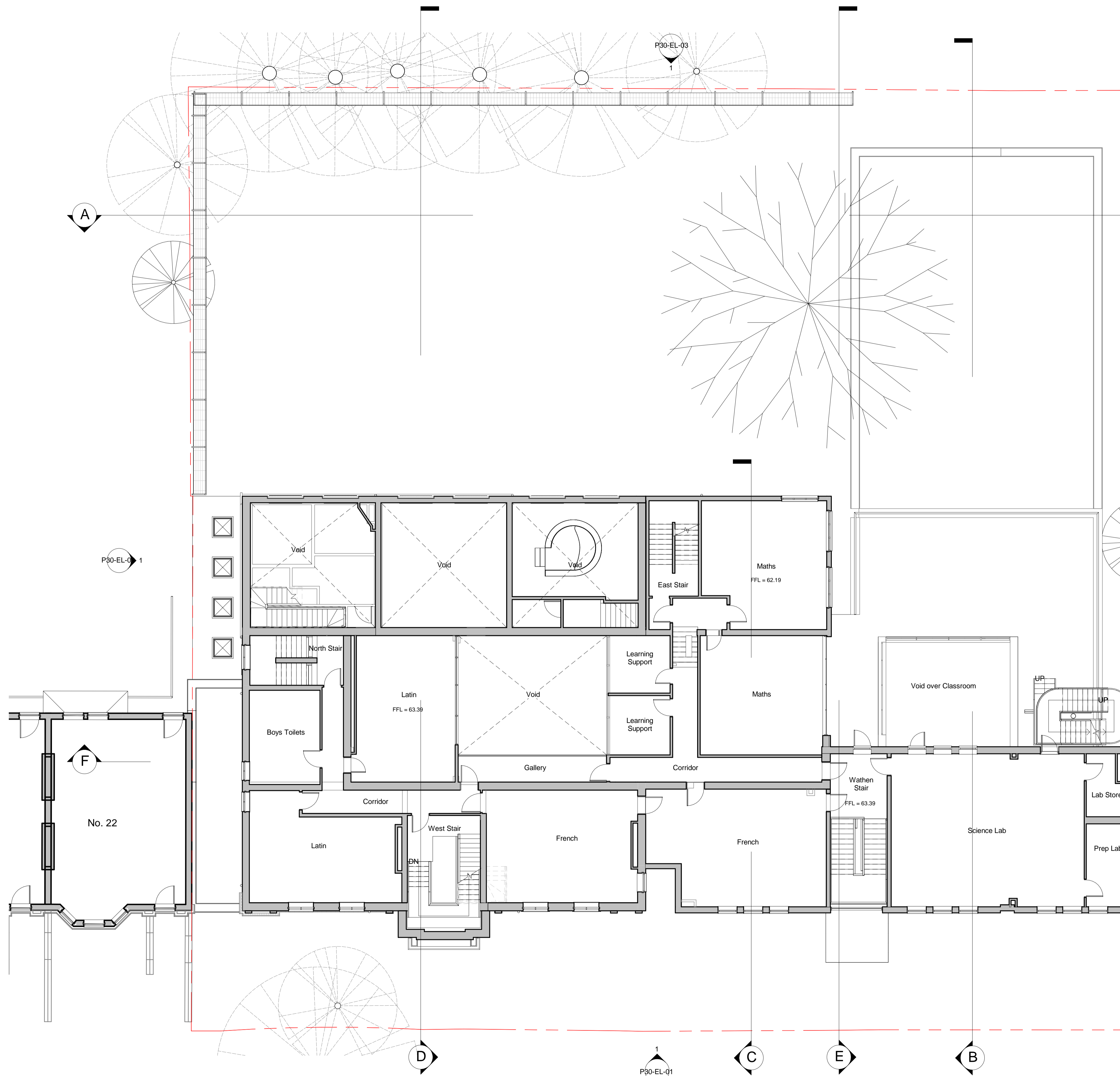
Existing L01 First Floor 1 : 100
