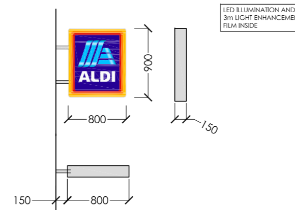
SIGN 6: ALDI PROJECTING SIGNCASE - 1:50
