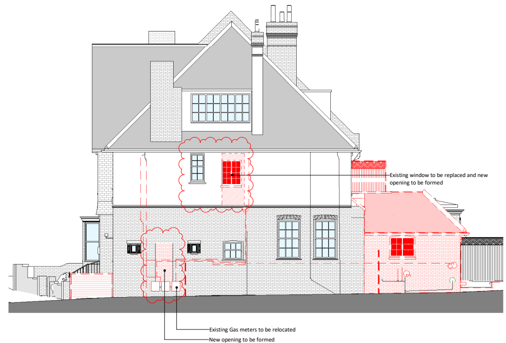
2 Demolition Side Elevation 1 : 100
