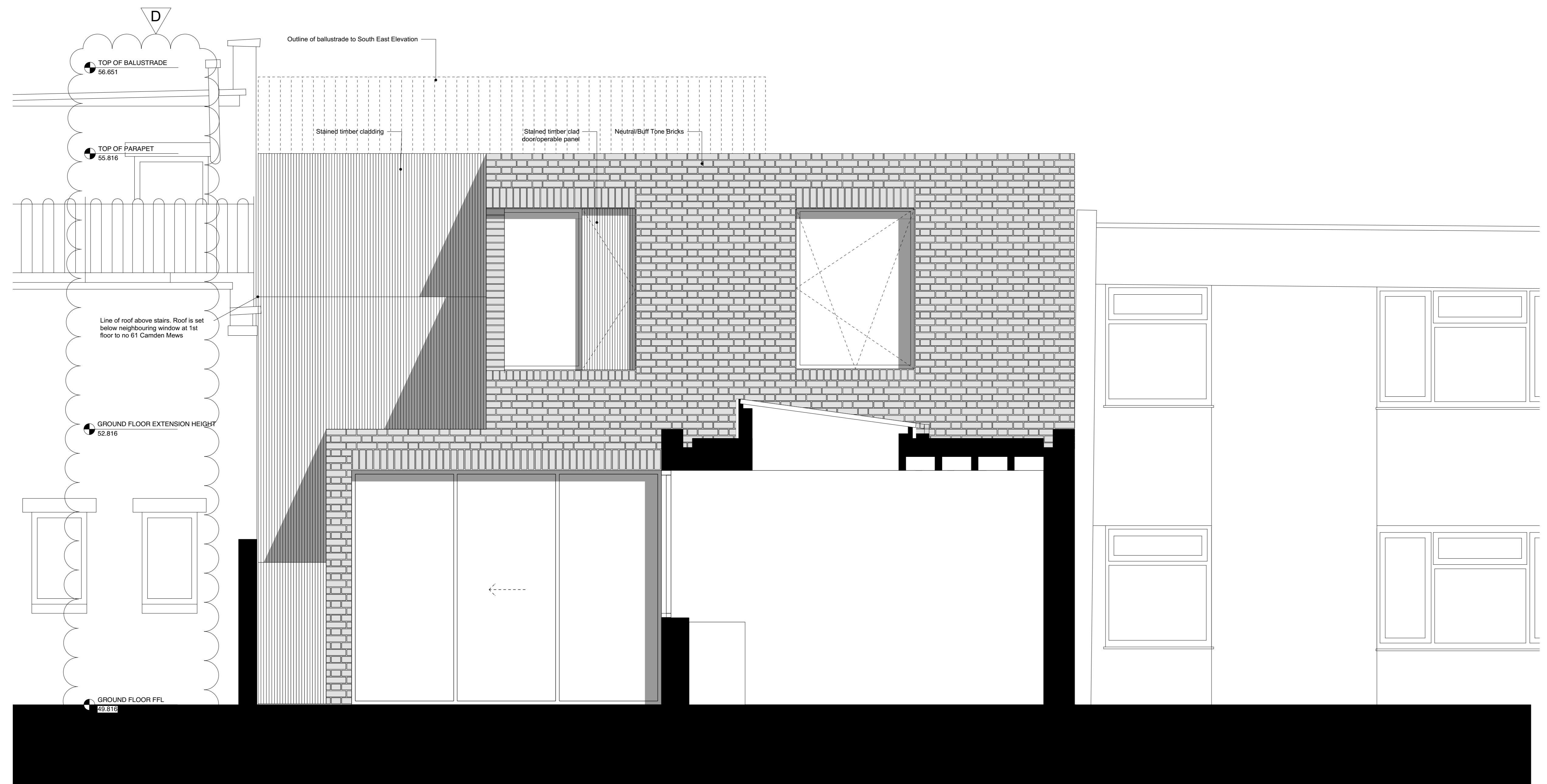
1 Proposed Elevation Along Camden Mews (NW) 1:25 @ A1
