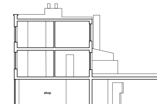
Existing Section AA Scale 1:100
