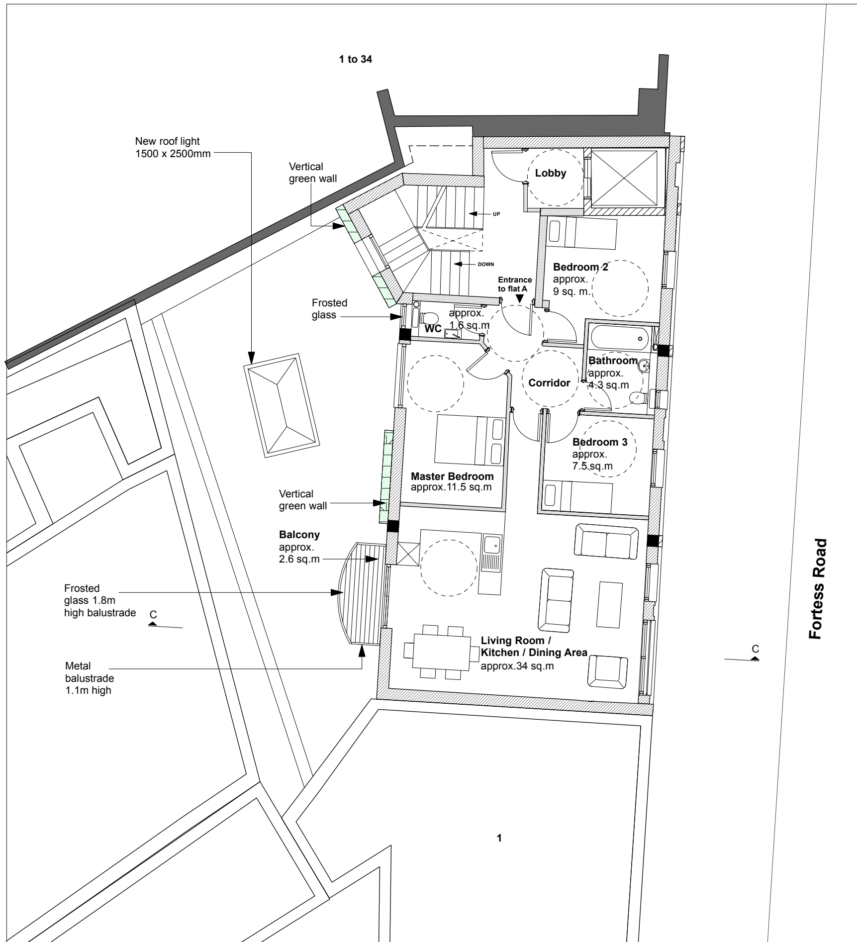
Proposed First Floor Plan Scale 1:100
