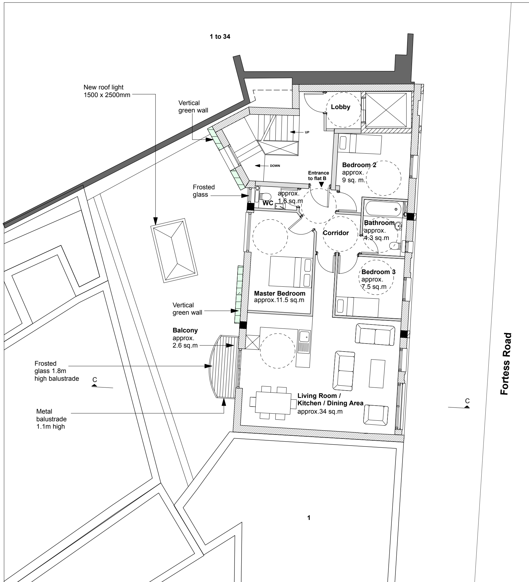
Proposed Second Floor Plan Scale 1:100
