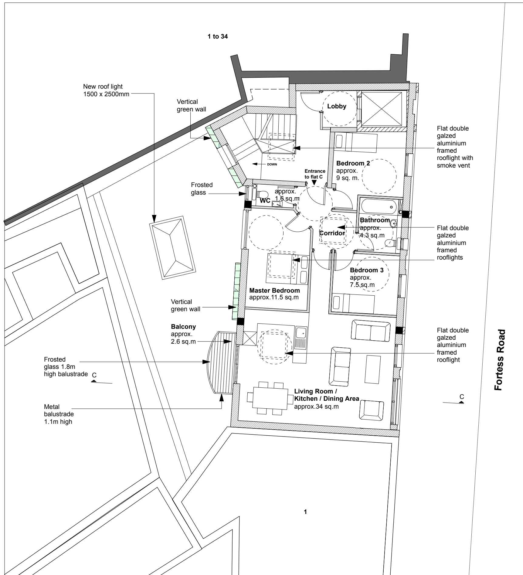
Proposed Third Floor Plan
