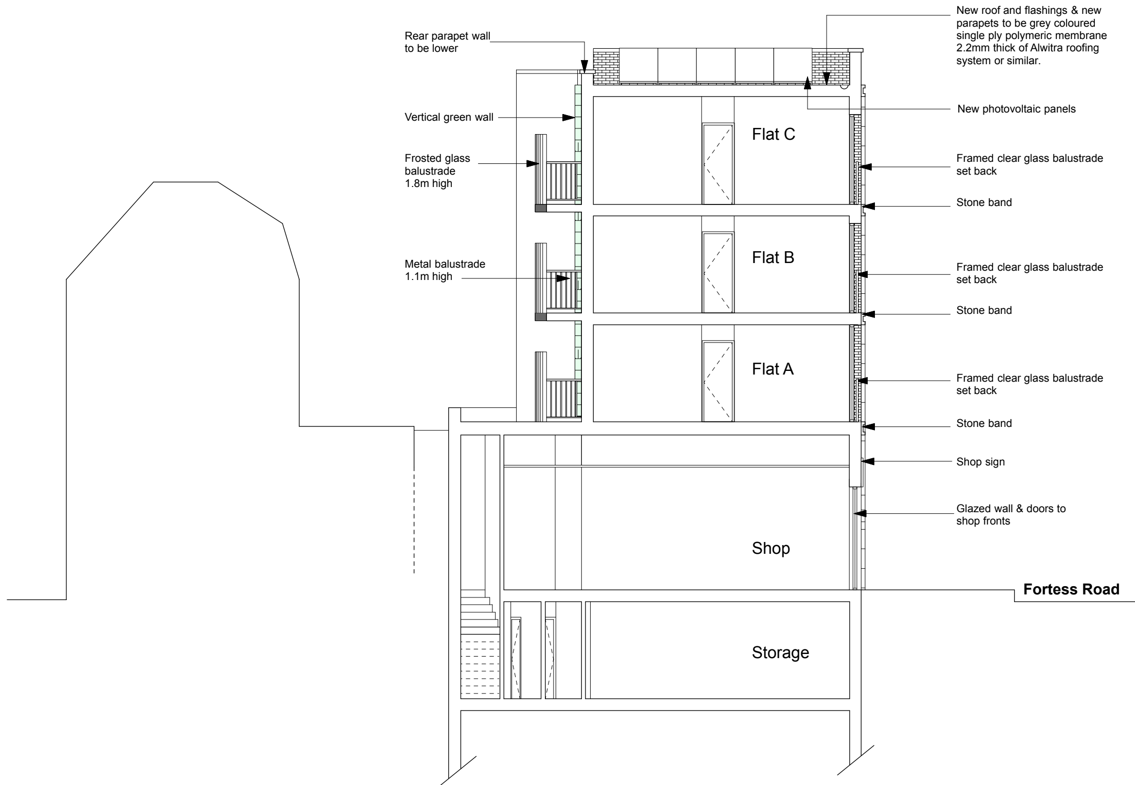
Proposed Section CC Scale 1:100
