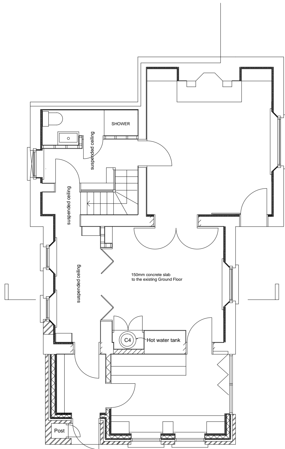
GROUND FLOOR
