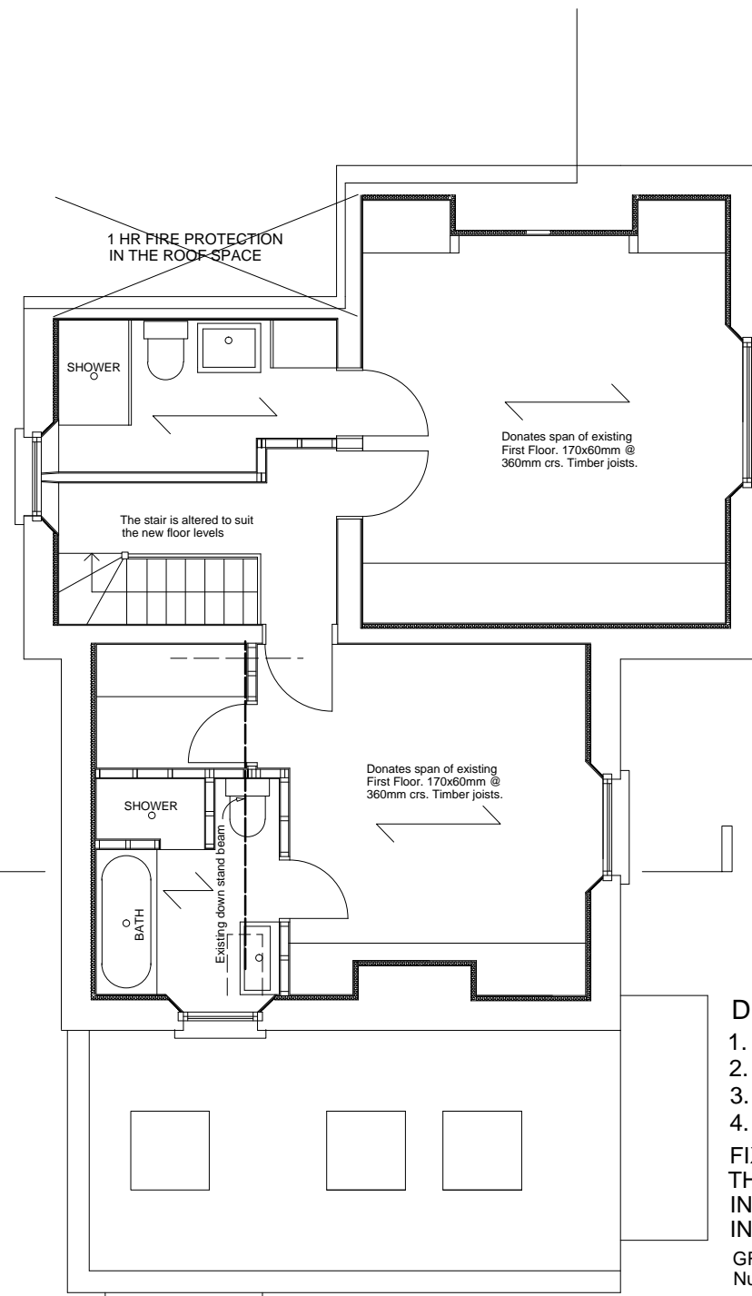
FIRST FLOOR
