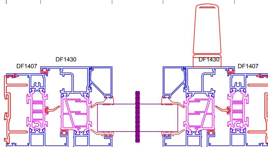
Horizontal section B-B (1:2)
