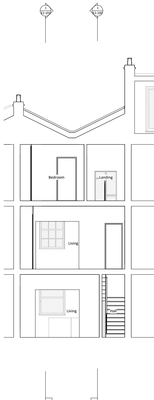
Section 3 1:50
