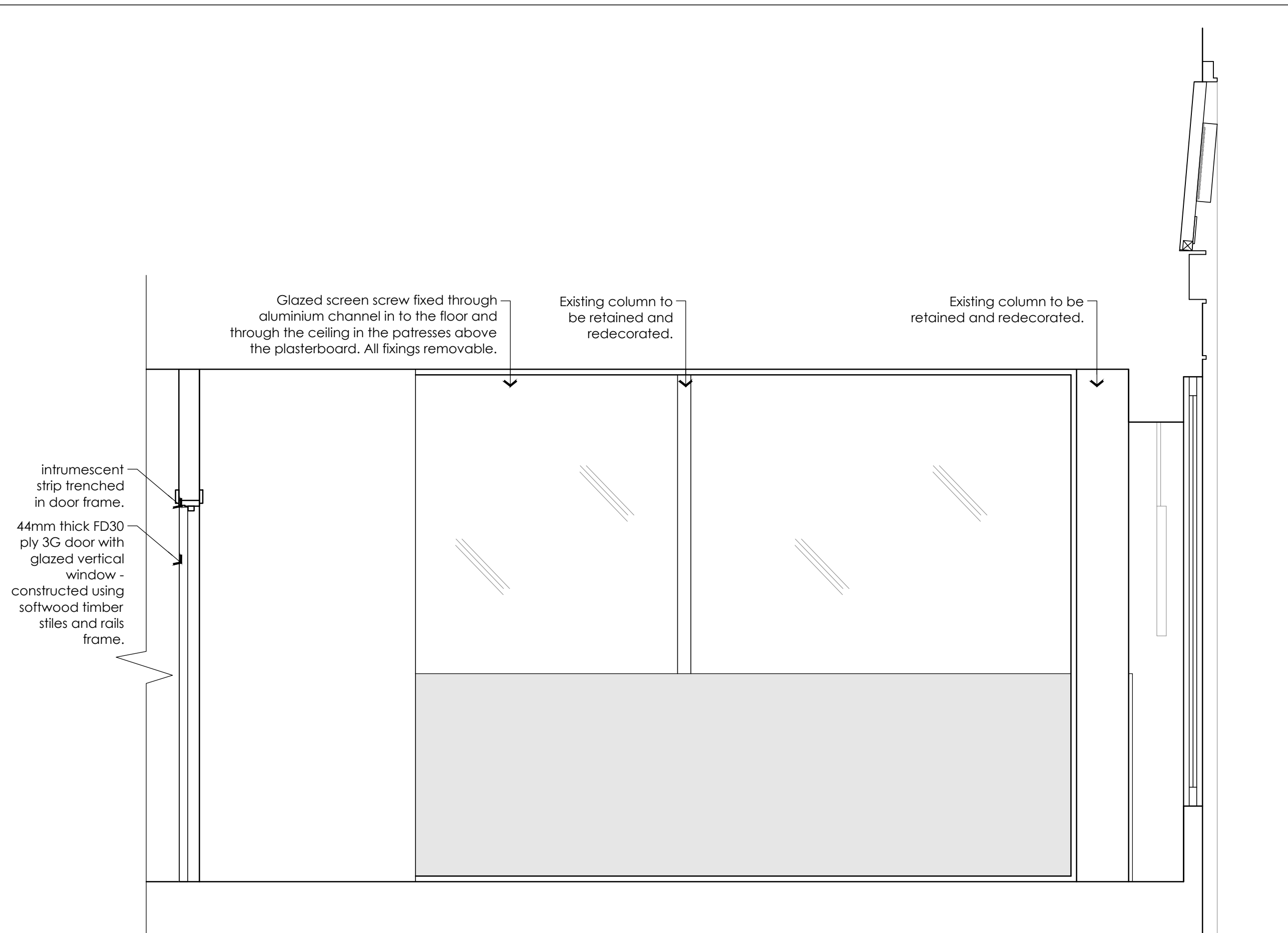
Internal Elevation A Proposed
