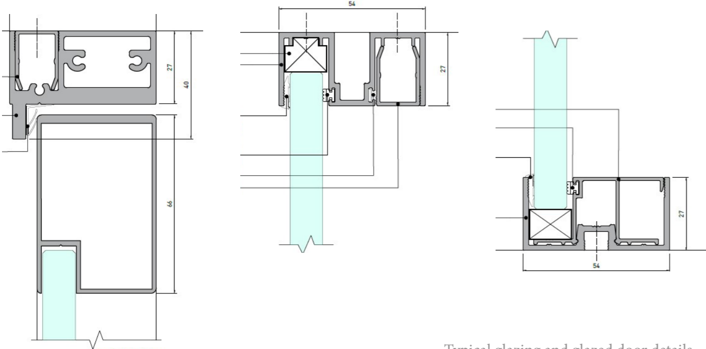
Typical glazing and glazed door details
