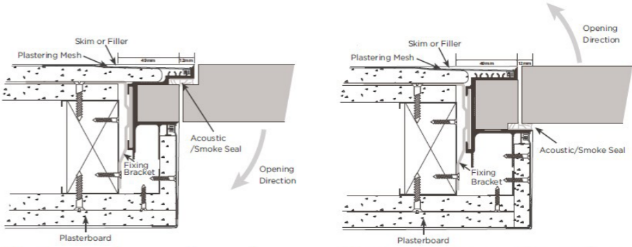
Typical door details
