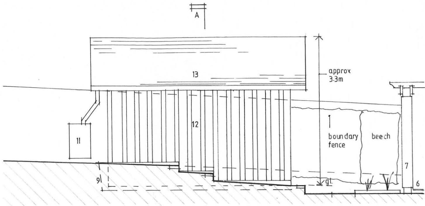
ELEVATIONS B [elevation E similar but handed]
