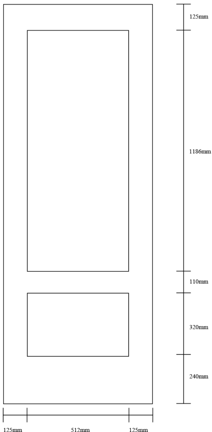
Low Mid-Rail 1981 x 762mm
