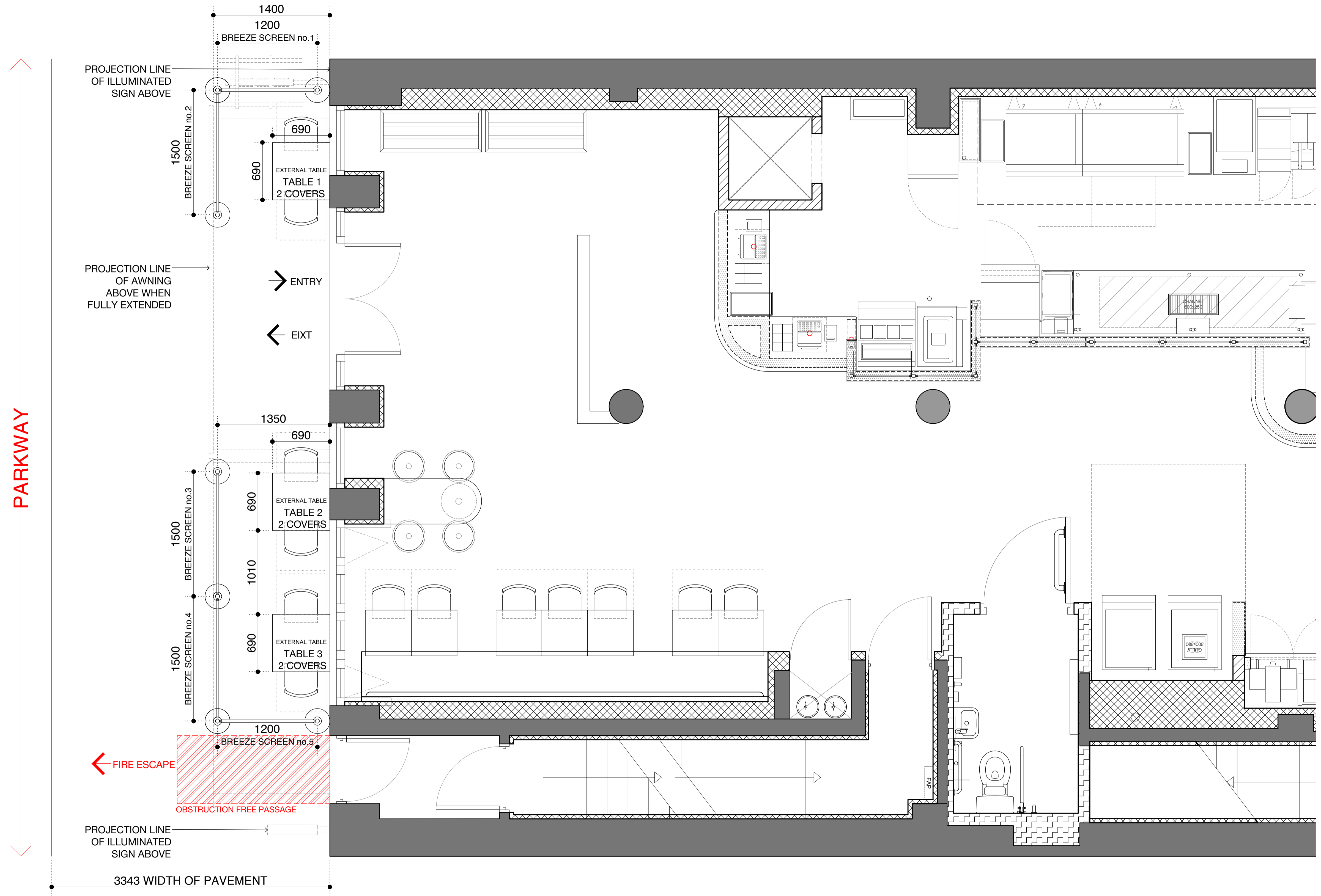
02 SHOPFRONT ELEVATION B - FULLY RETRACTED AWNING SCALE 1:50 @ A3
