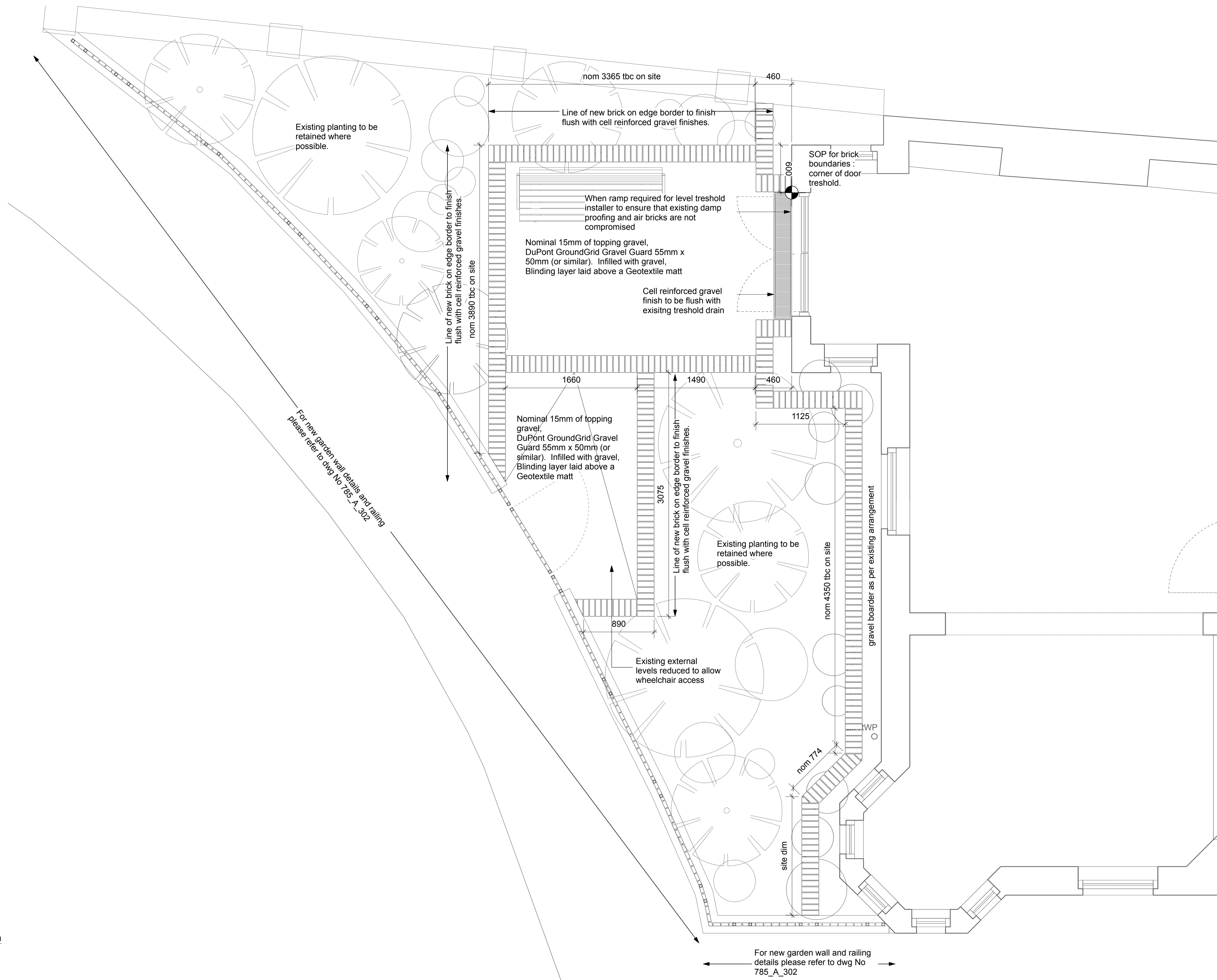
1 Front Garden Plan Scale: 1:25
