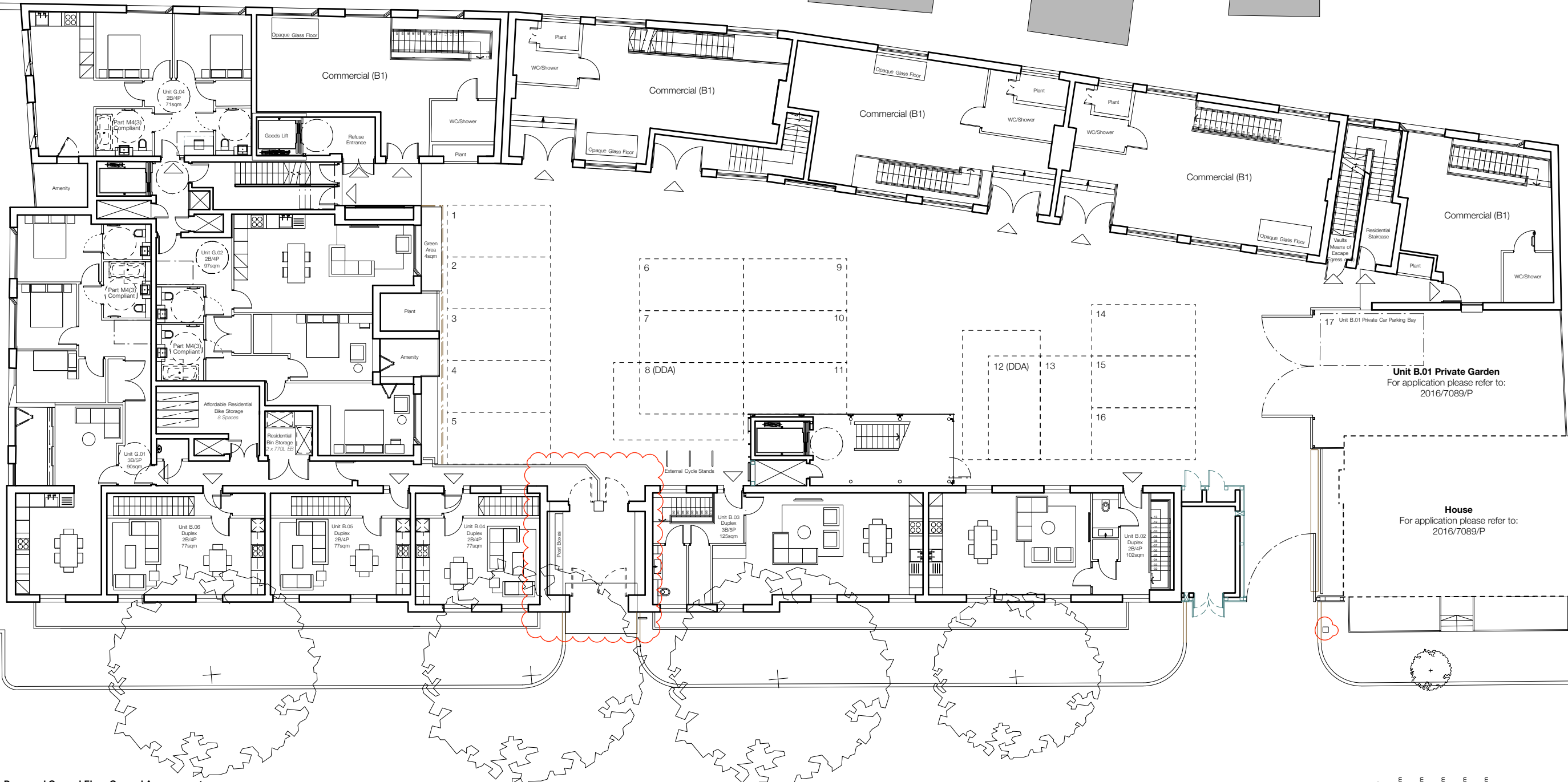
A Proposed Ground Floor General Arrangement GA.00 1:100 @A1 1:200 @A3
