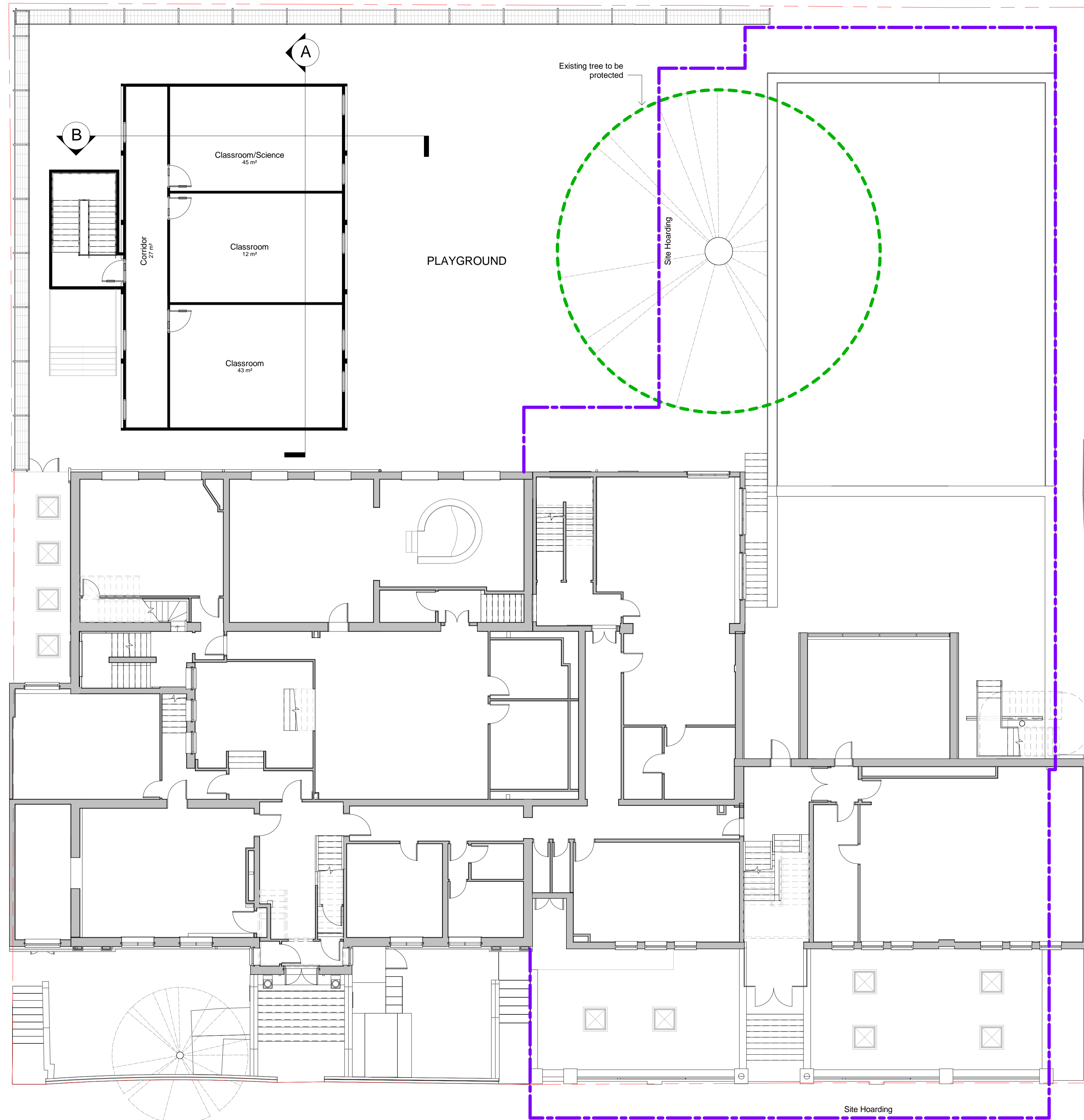
TEMPORARY ACCOMMODATION - FIRST FLOOR 1 : 100
