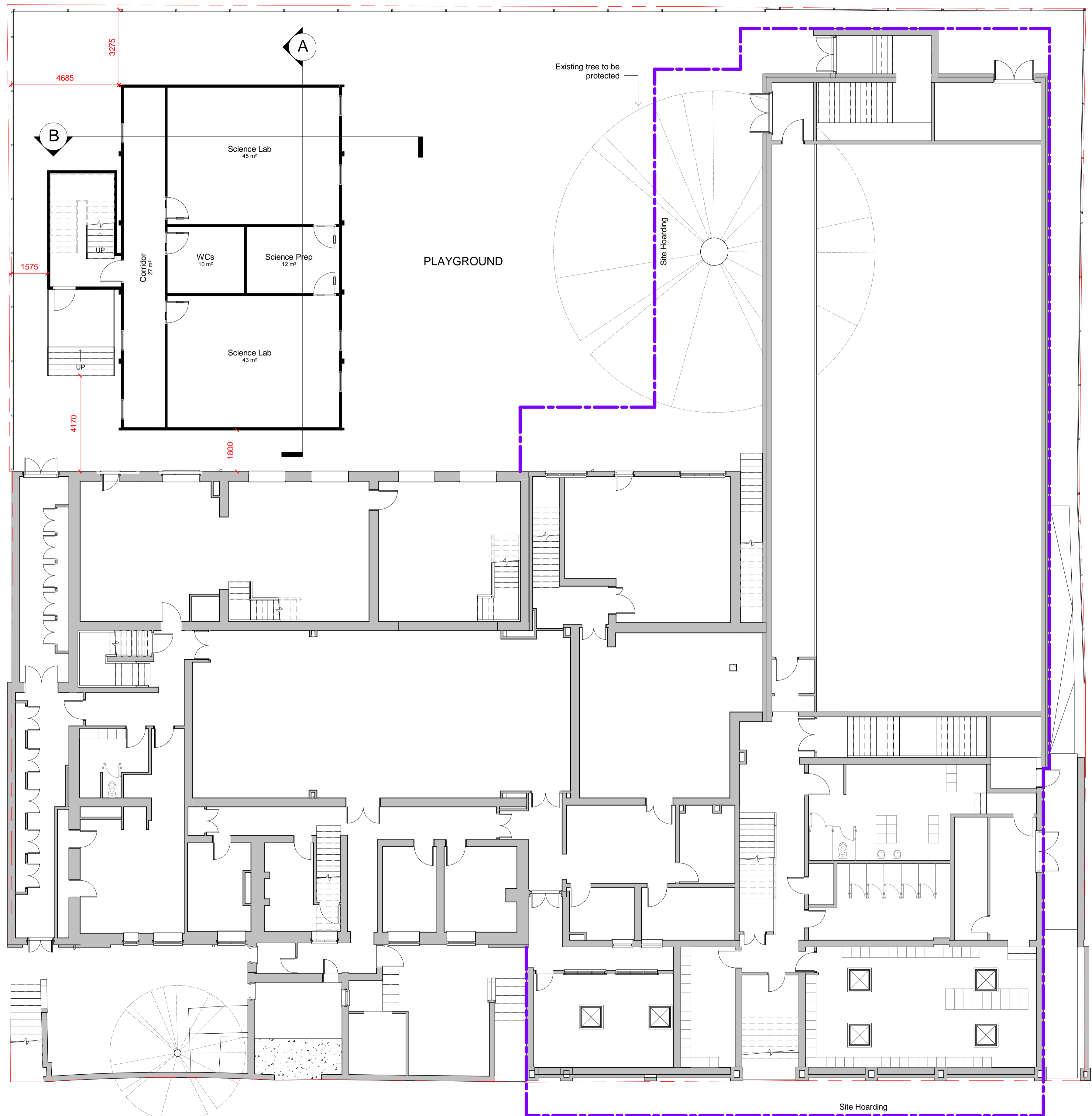
TEMPORARY ACCOMMODATION - GROUND FLOOR 1 : 100
