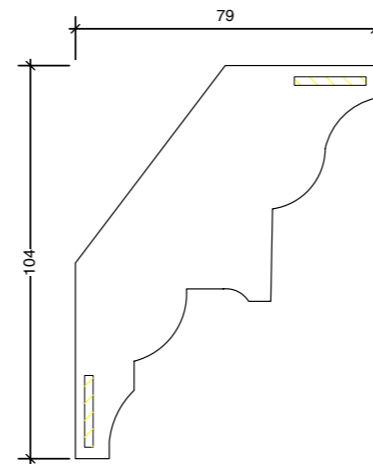
PROPOSED CORNICE FOR MASTER DRESSING 1 & 2, BEDROOMS 2, 3 & 4
