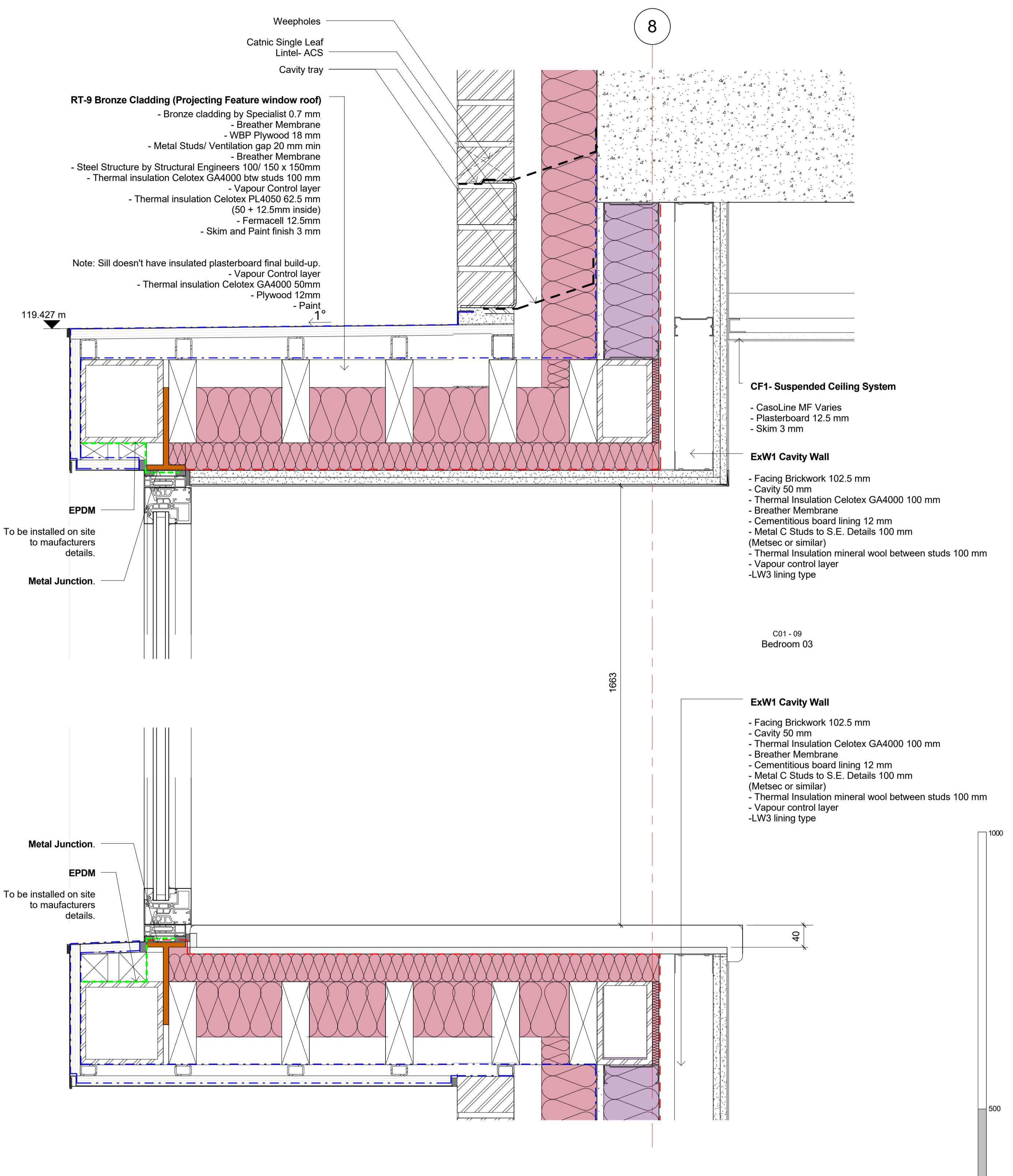
2 CORNER BAY WINDOW - SECTION 1 : 5
