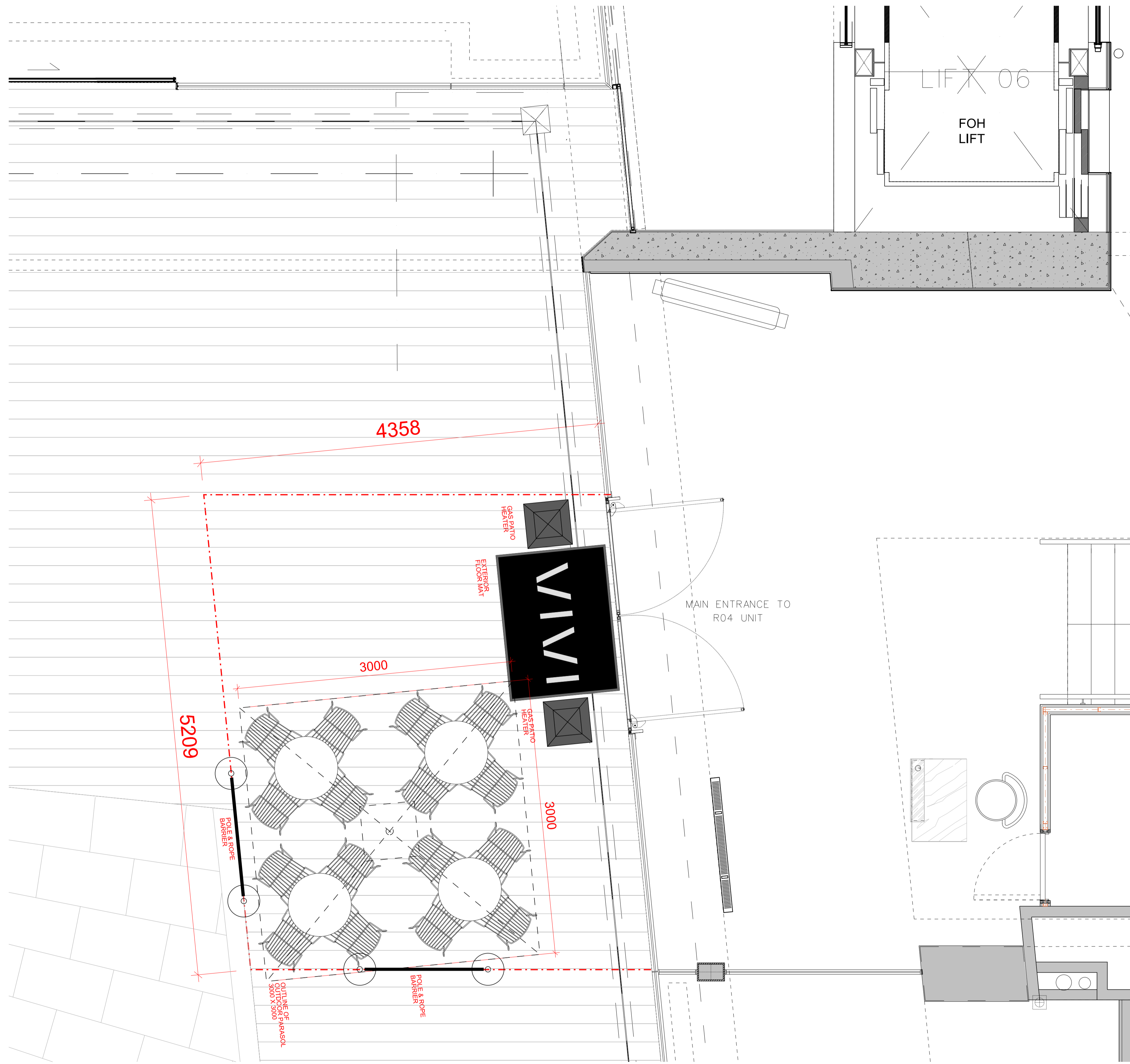
① LEVEL 00 - PLAN PROPOSED 1:25
