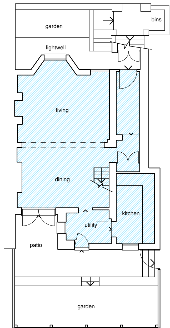
Existing ground floor plan Scale 1:100 @A3
