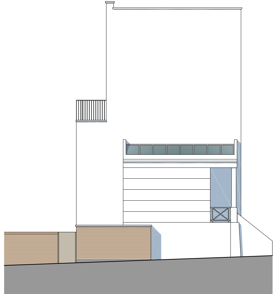
Existing side elevation Scale 1:100 @A3
