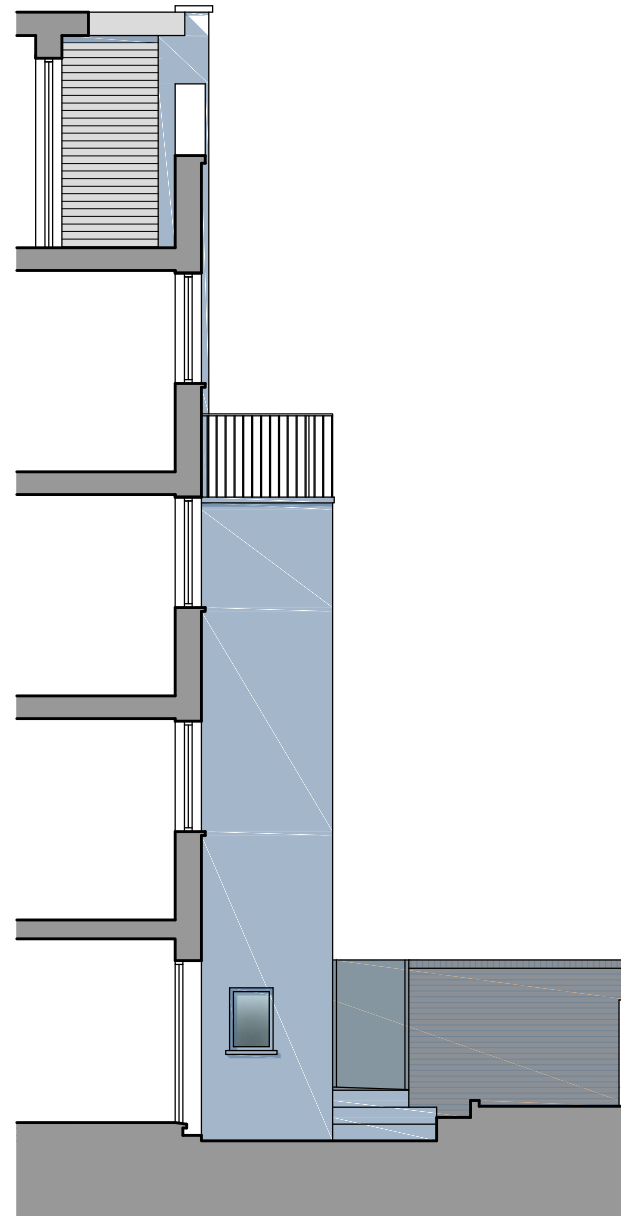
Existing side elevation/ part section Scale 1:100 @A3
